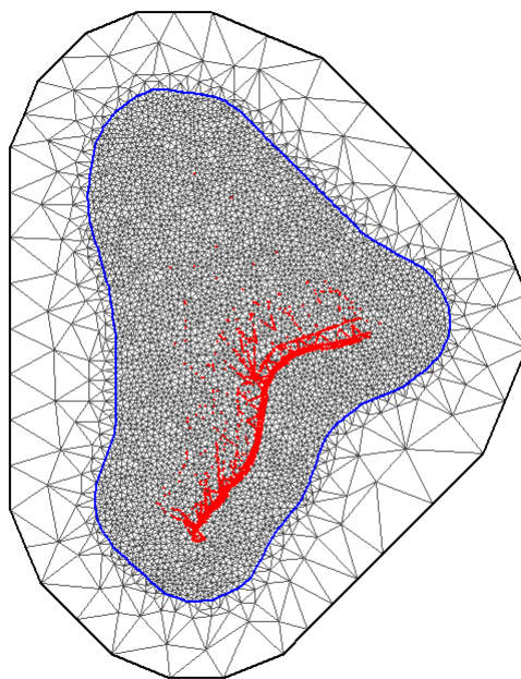
Constrained refined Delaunay triangulation
