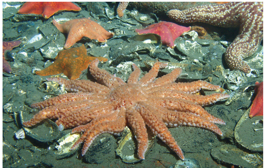
Figure 4. Shell mounds accumulate on formerly soft bottoms under oil platforms off California change the nature of the benthic habitat and attract a different community of organisms, including the seastars shown here and fishes (Goddard and Love, 2008). Donna Schroeder, Minerals Management Service
