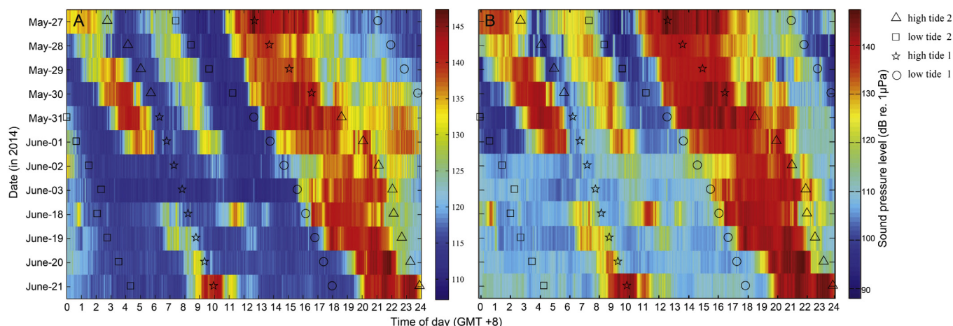
Fig. 13. Timing of tidal phases compared to the temporal patterns of (A) broadband sound pressure levels ( SPL_{rms} ) and SPL_{lfb} (B) as a function of the time of day (X axis) and date (Y axis). For semidiurnal tidal conditions, the peak tidal phase generally includes the first and secondary high tide periods. The valley tidal phase generally covers the first and secondary low tide period.
