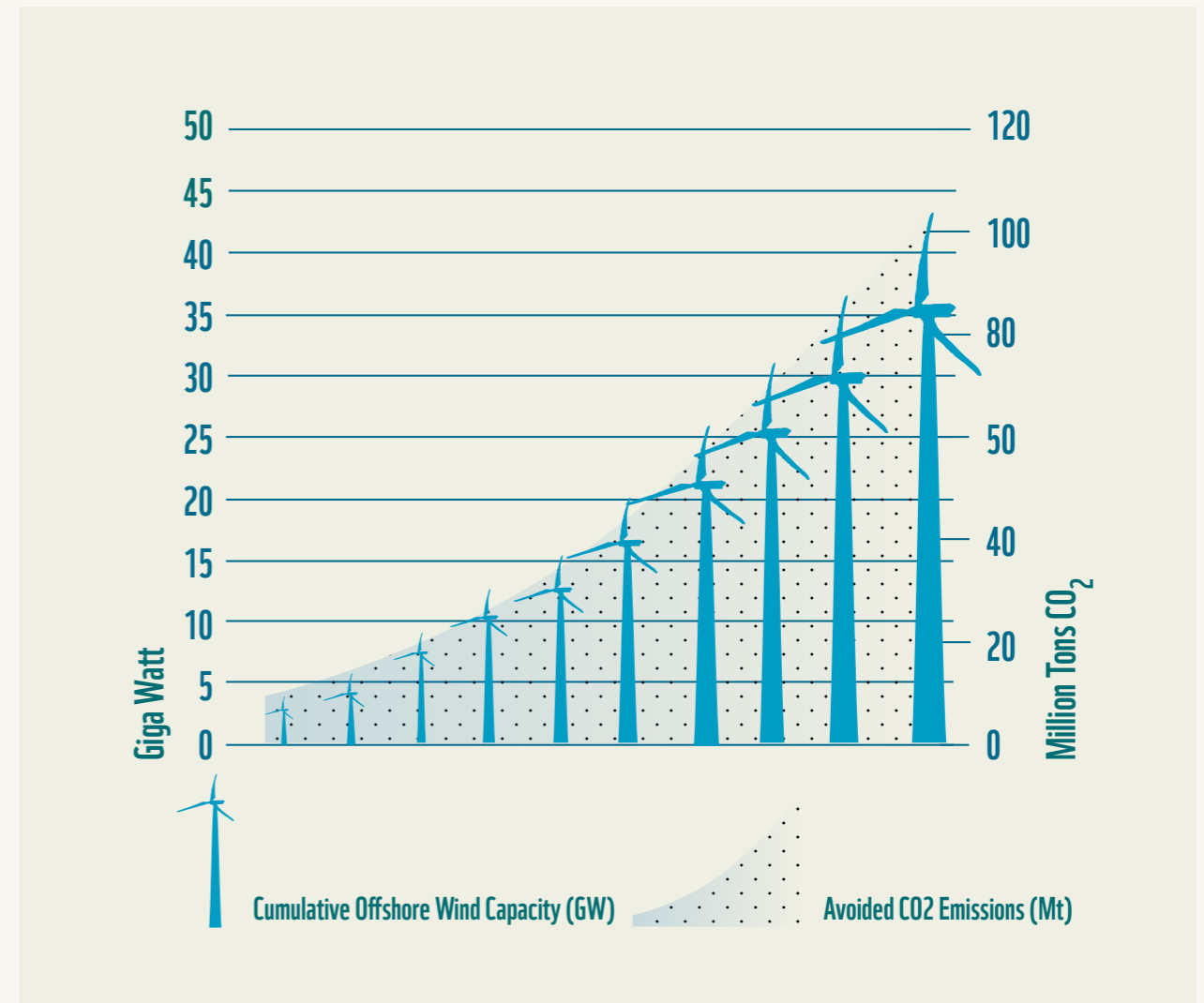
In 2011, offshore wind power avoided the emissions of 9.8 million tons of CO 2 . Assuming the projected increase of installed capacity is realized, offshore wind will avoid 102.1 million tons of CO 2 in 2020. This reduction constitutes nearly twice the amount of Norway's yearly GHG emissions 16 .
