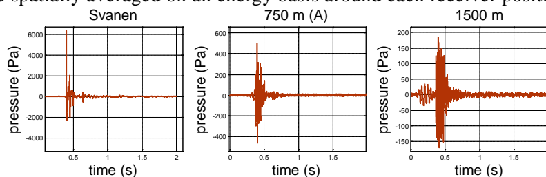
Figure 2 – Example of received acoustic pressure from air-gun shots (Pa vs. s) at P02 site: at the Svanen, 750 m (A) and 1500 m stations. Hydrophone depths are 2.5-3 m off bottom. Air-gun depth is at depth 7.5 m.
