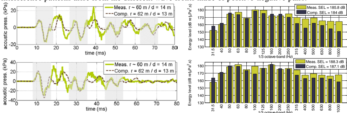
Figure 7 - Results of the WEAP-FE method at P23 site, Anholt OWF: measured vs. computed hydrophone time series and 1/3-octave energy spectra for a penetration depth of 10.1 m (top) and 18.1 m (bottom). Numerical receiver range and depth are identical for both FE runs and are within +/-2 m from the measured ones. Grey regions correspond to the odd phase numbers in (1).
