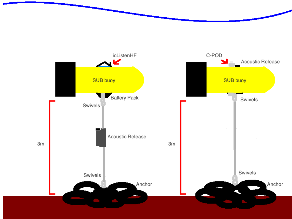
Figure 10. Specialized SUB buoy mooring designs for the icListenHF hydrophone (left) and the C-POD deployments (right). Mooring components shown are not to scale.
