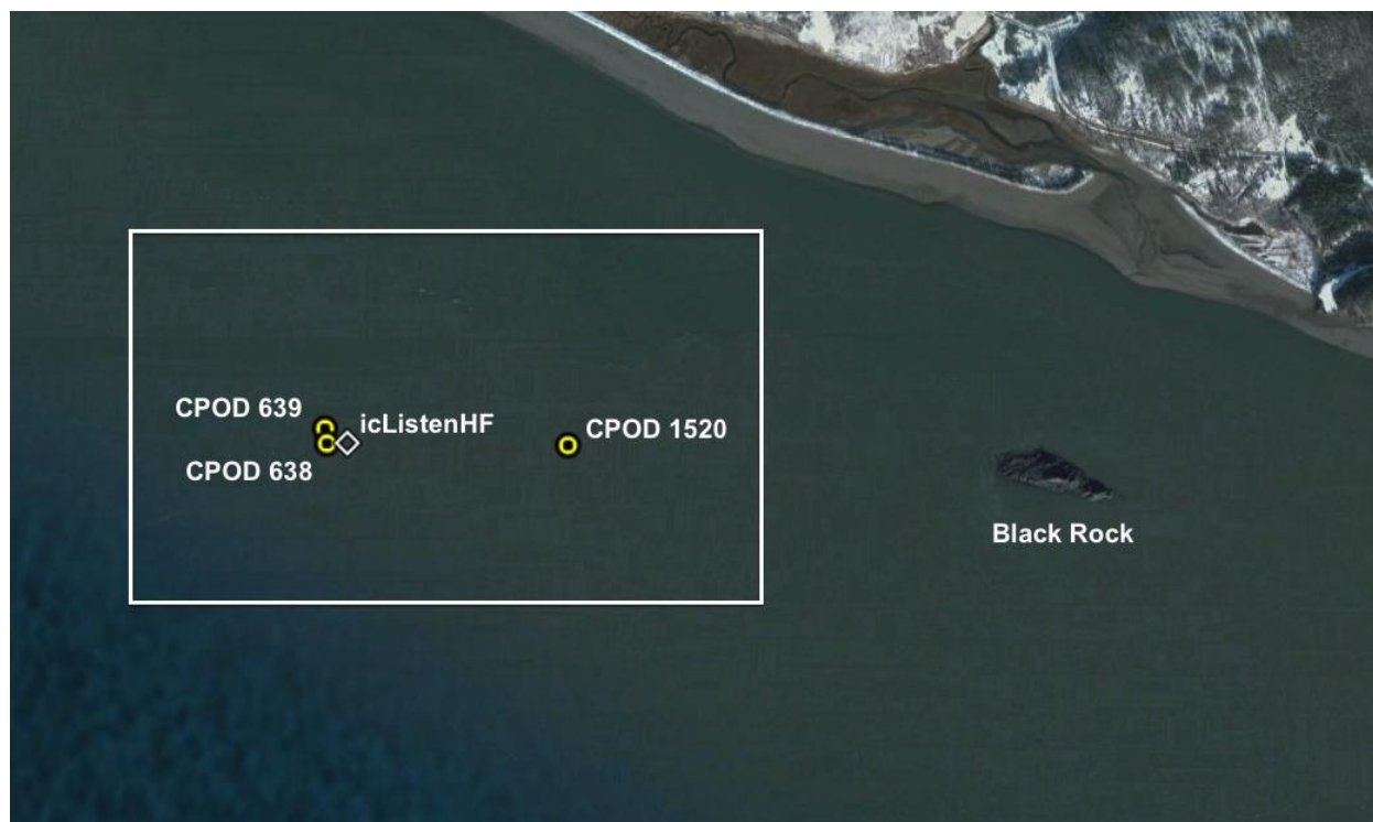
Figure 11. Locations of C-POD and icListenHF hydrophones deployed on August 1st 2012 within the FORCE test site (1 km x 1.6 km).
