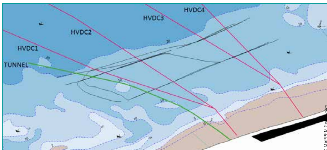
Fig. 8: Positions of the transects defined using the PASSEM tool (black lines) to measure the electromagnetic fields emitted by the cables of the HVDC Cross-Channel interconnector (red lines).
