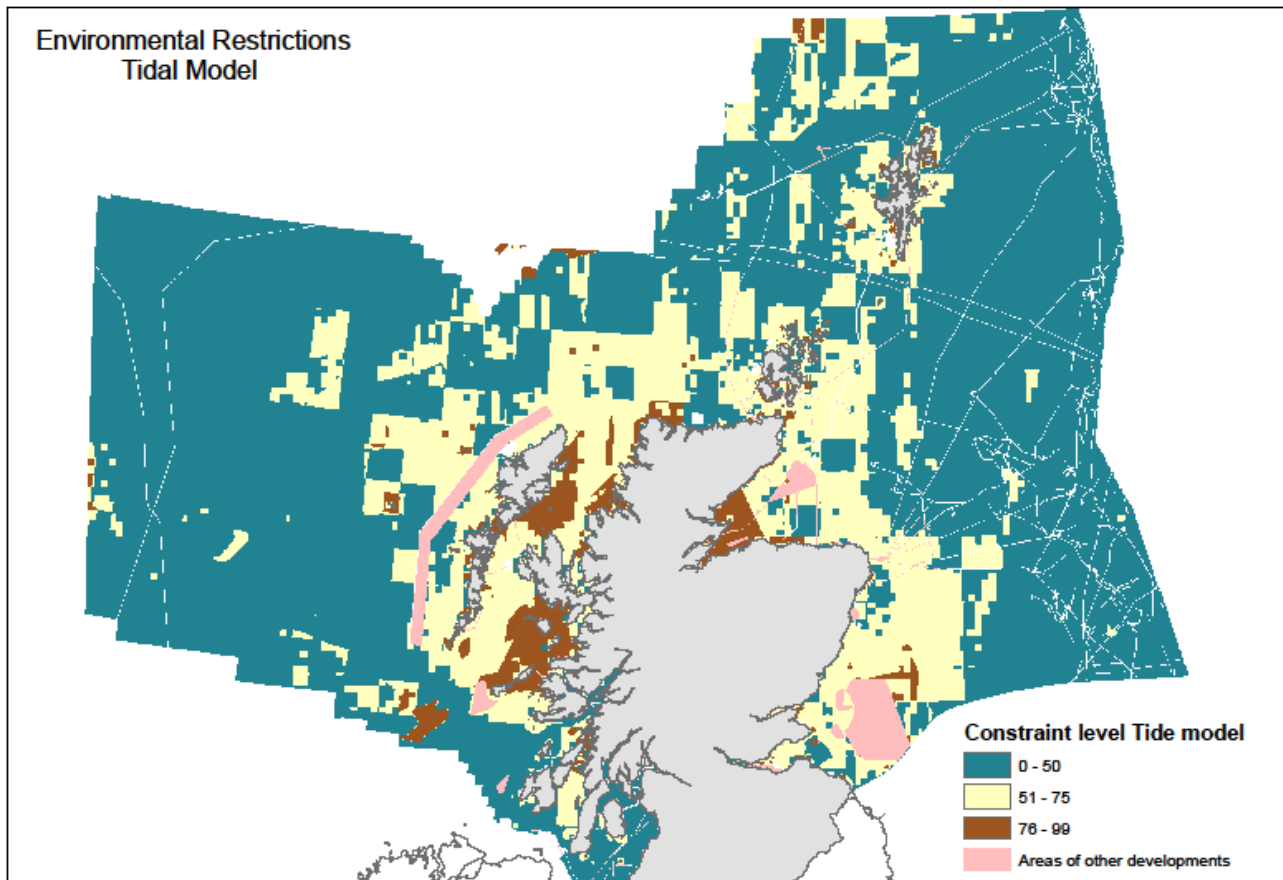
Figure A1.2 Environmental risk map for tidal stream energy projects, showing areas of low (green), medium (yellow) and high (brown) environmental risk.
