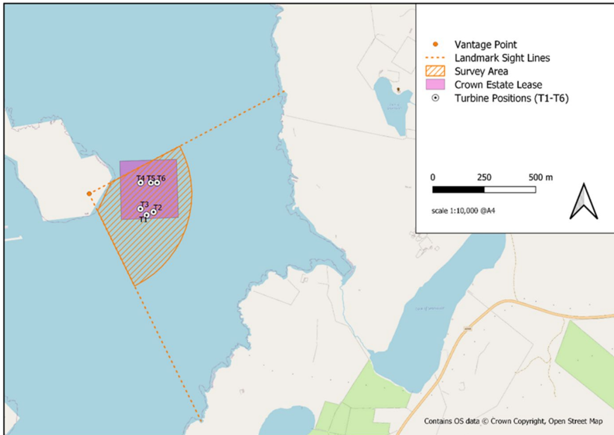
Figure 3-1 Land-based survey area in Bluemull Sound, showing locations of the four installed turbines (T1 to T4) and locations of turbines in the expanded array (T5 to T6).
