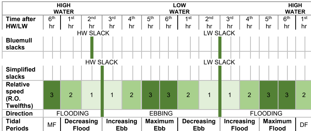
Figure 3-2 The six tidal periods within the tidal cycle during which land-based surveys are conducted.
