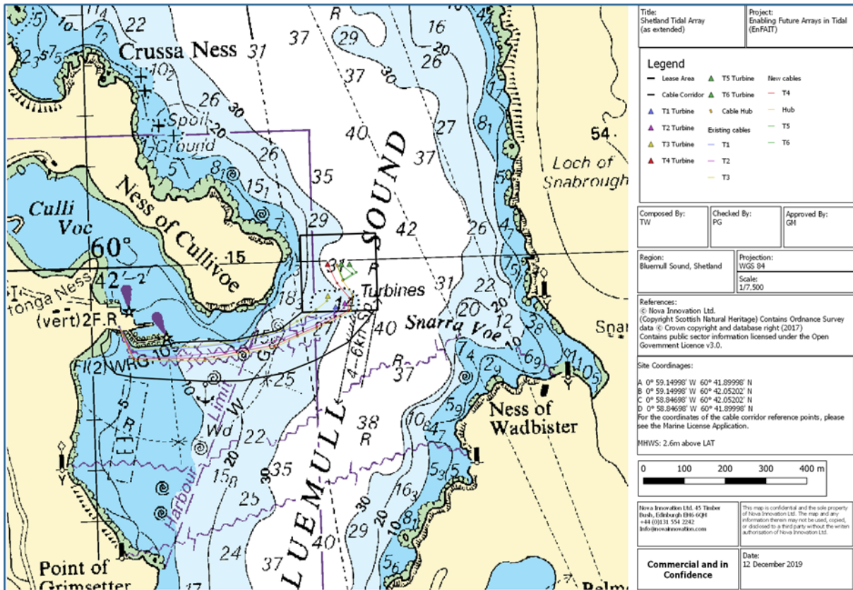
Figure 2-3 Shetland Tidal Array layout (Admiralty Chart). Source: Nova Innovation 2020 © Crown Copyright
