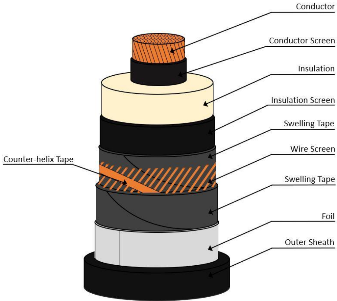
Figure 3.3-15 Representative Cross-Section of Onshore Export Cable
