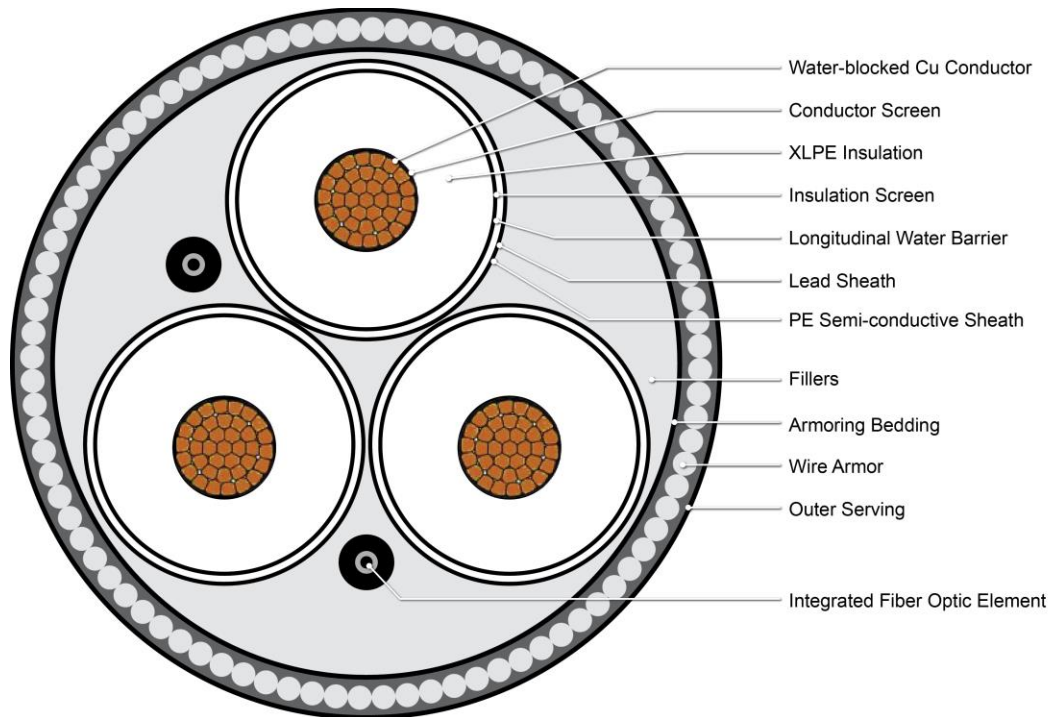
Figure 3.3-6 Representative Cross-Section of Submarine Export Cable
