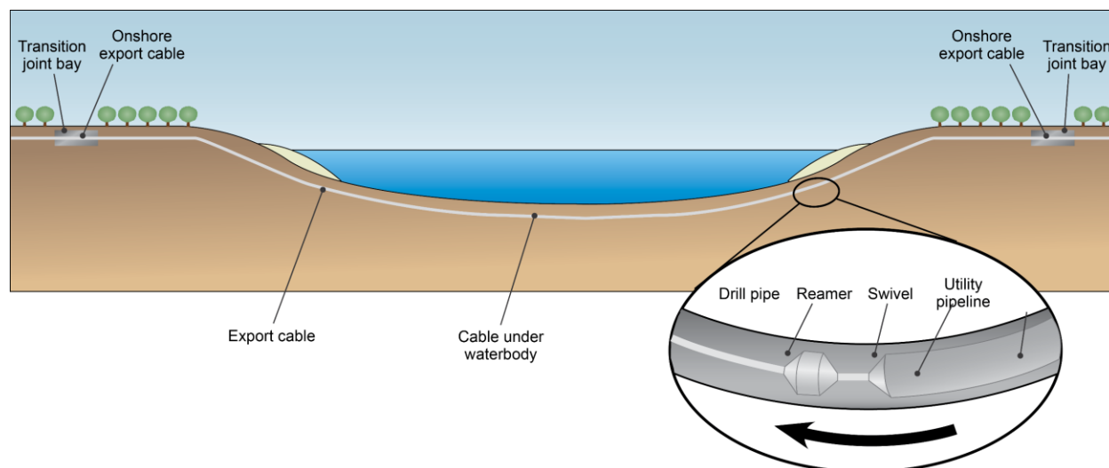
Figure 3.4-5 Onshore Crossing HDD
