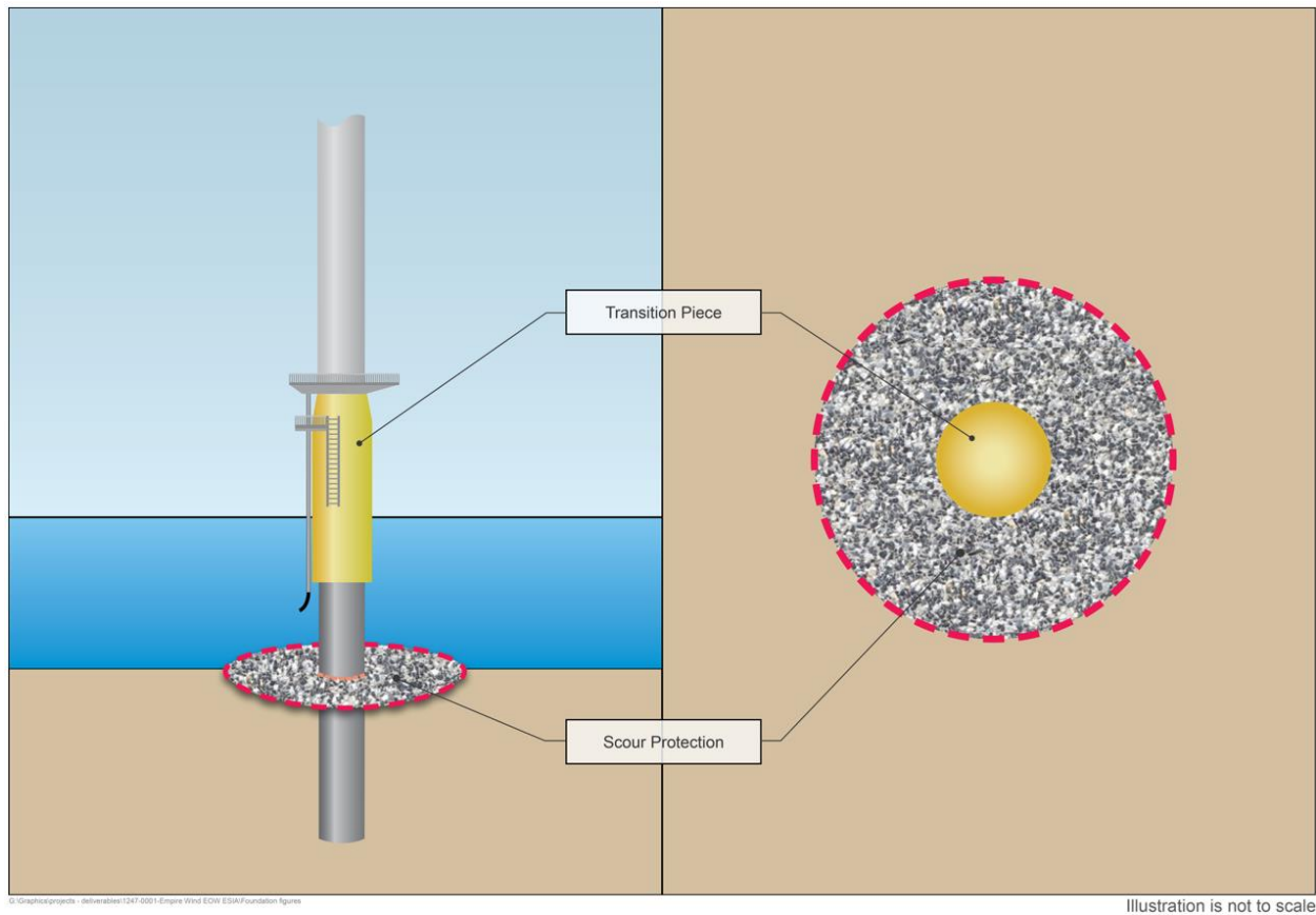
Figure 3.3-10 Example of Scour Protection Installation for Monopile Foundation
