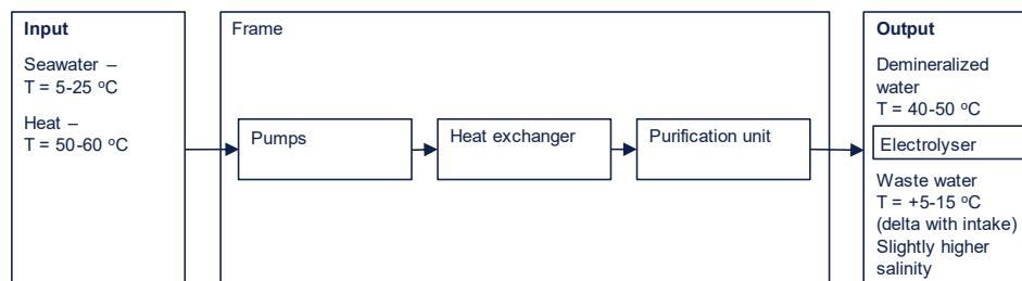
Figure 0-2 Schematics for platform concept, hydrogen production on an offshore platform.
