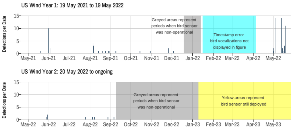
Figure 8. Daily bird occurrences at the E14 US Wind buoy during collection period 19 May 2021–10 January 2023. This figure does not include the 43 birds recorded during the period when accurate timestamps were missing.
