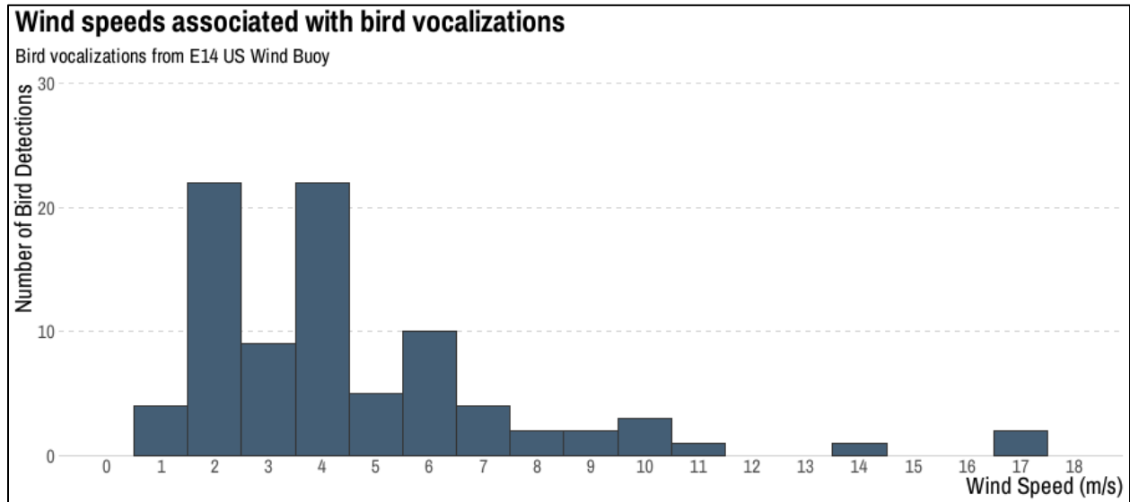
Figure 9. Bird acoustic detections recorded per wind speed (m/s) at the US Wind Buoy E14 . This figure does not include the 43 birds recorded during the period when accurate timestamps were missing.
