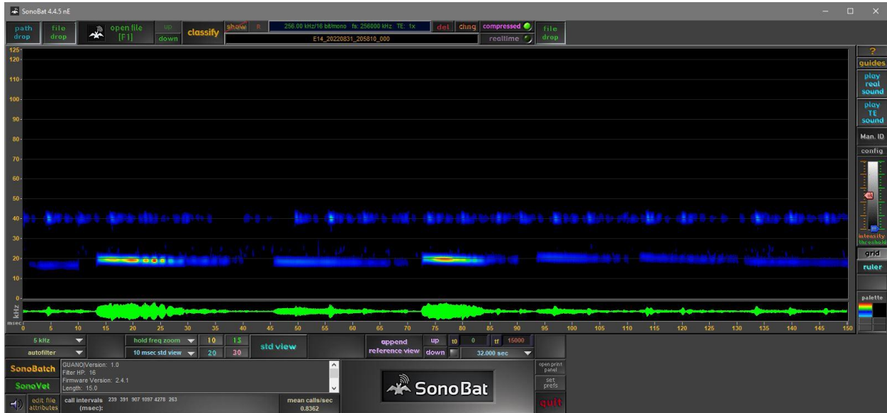
Figure 6. Spectrogram of hoary bat collected at the E14 US Wind buoy.
