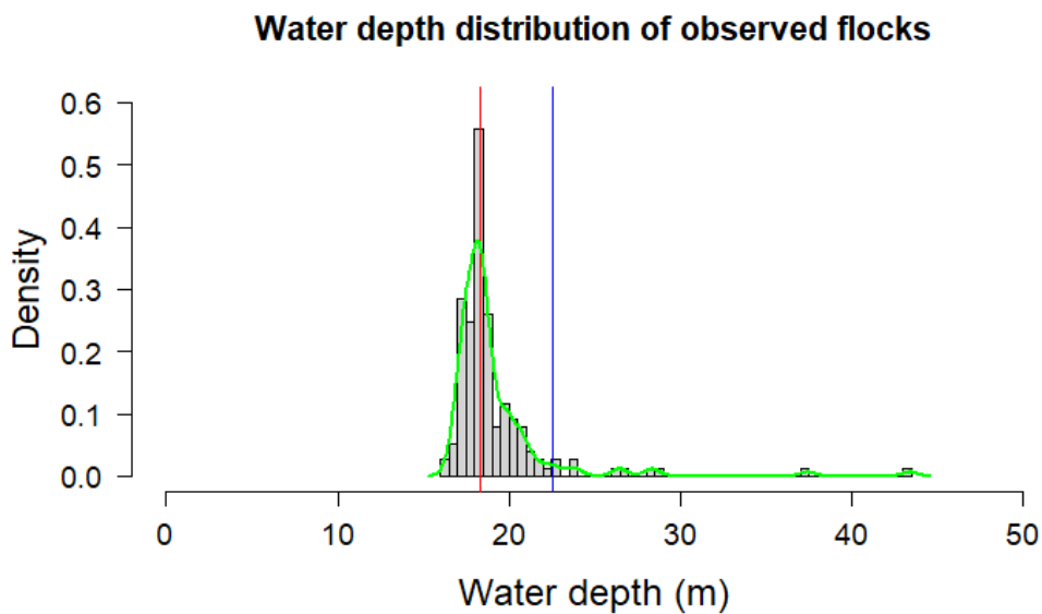
Figure 11 – Water depth distribution of Long-tailed Duck observations during the 2022/2023 surveys. The red vertical line indicates the median water depth at which Long-tailed Ducks were observed and the green curve is the probability density line of the distribution. The blue vertical line indicates the median water depth in the survey area.
