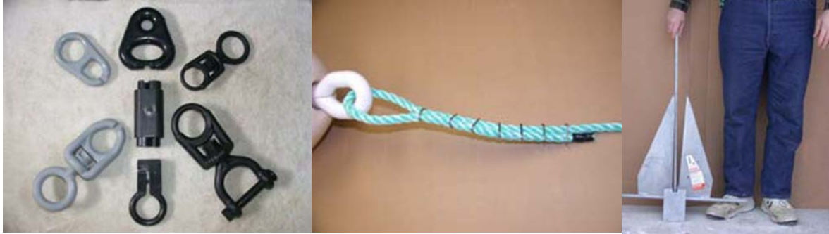
Figure 11. Gear modifications for fixed gear as part of the ALWTRP on the U.S. east coast to reduce whale entanglements: weak links and modified anchors.
