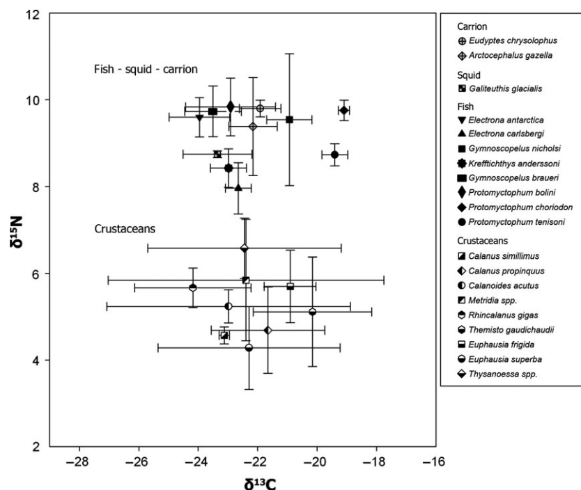
Fig. 6. Mean \delta^{15}\text{N} and \delta^{13}\text{C} ( \pm\text{SD} ) in 20 species of crustacean, fish, squid and carrion (fur seals Arctocephalus gazella and Macaroni penguin Eudyptes chrysolophus ) sampled in four locations within the birds' foraging distribution at sea that differed greatly in temperature, productivity and nutrients (Stowasser et al. 2012).
