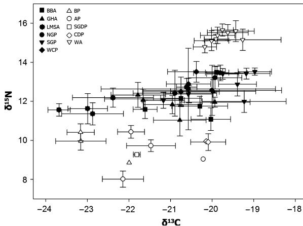
Fig. 5. Mean \delta^{15}\text{N} and \delta^{13}\text{C} ( \pm\text{SD} ) in feathers of chicks of 11 procellariiform species (WA, wandering albatross; BBA, black-browed albatross; GHA, grey-headed albatross; LMSA, light-mantled sooty albatross; INGP, northern giant petrel; SGP, southern giant petrel; WCP, white-chinned petrel; BP, blue petrel; AP, Antarctic prion; SGDP, South Georgia diving petrel; CDP, common diving petrel) sampled at Bird Island, South Georgia, during several years covering a 13-year period.
