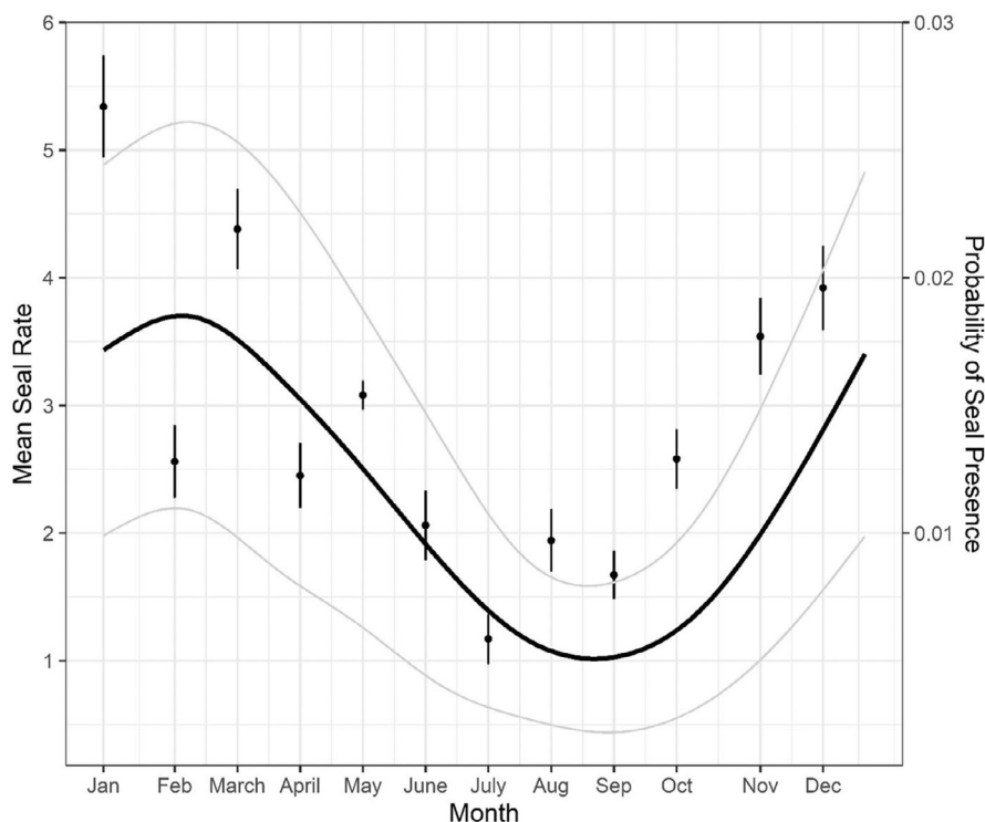
FIGURE 2 Daily mean seal rates per month ( \pm standard error) overlaid by a GAM plot displaying the predicted probability of seal presence in a 10-min bin across the year, with a smooth (95% CI defined by grey lines). Median value for hour = 12, median value for speed = 1.9 \text{ ms}^{-1} , across all auditors and operational status = 0.
