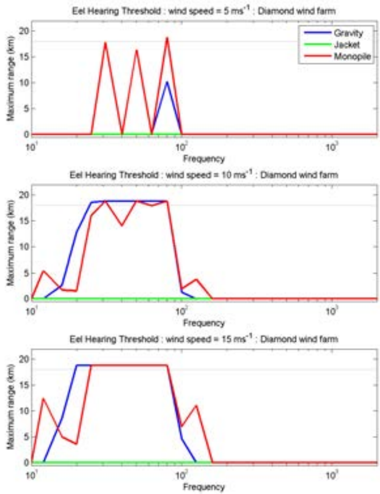
Figure 5-9 - Maximum range at which a European eel could hear a wind farm at different wind speeds. Gravity base, jacket and monopile foundations are compared. It is assumed that if the SPL is below the background noise that an eel could not hear the wind farm. The range is measured to the centre of the wind farm.
