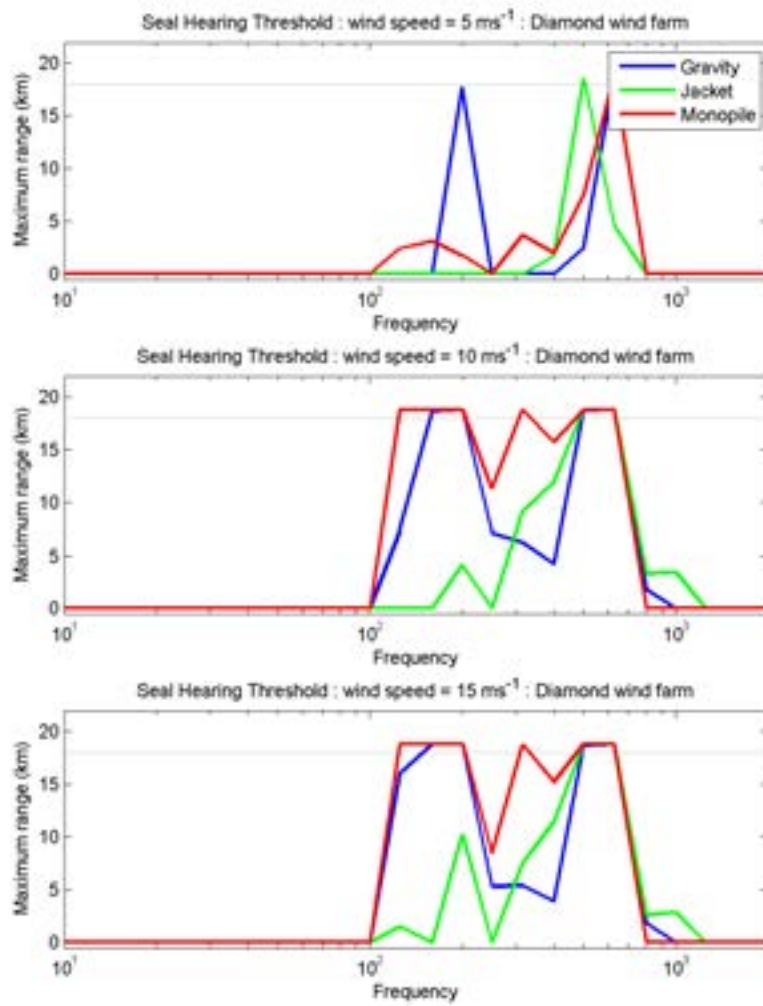
Figure 5-2 – Maximum range at which a harbour seal could hear a wind farm at different wind speeds. Gravity base, jacket and monopile foundations are compared. It is assumed that if the SPL is below the background noise that a seal could not hear the wind farm. The range is measured to the centre of the wind farm.
