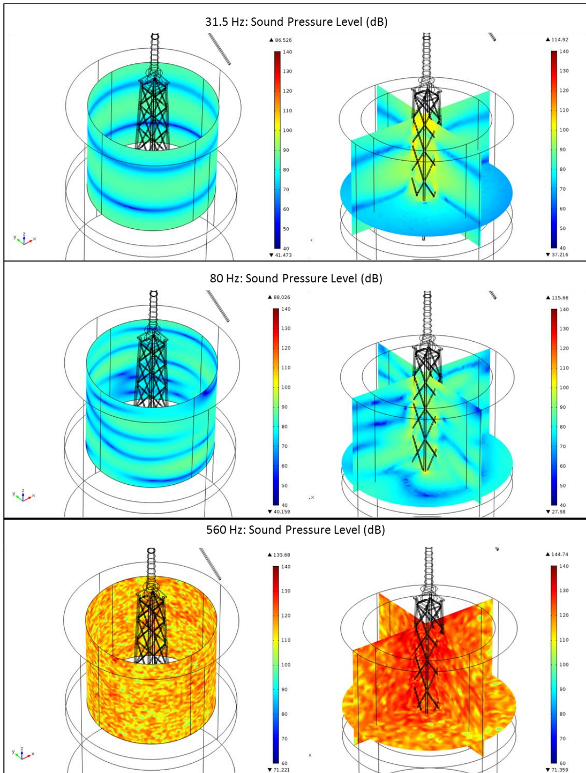
Figure 3-21 Acoustic soundscape from the jacket foundation for 31.5, 80 and 560 Hz at 15 \text{ ms}^{-1} . The lower frequencies exhibit the cylindrical spreading. The more complex lattice structure produces a noisier soundscape at the higher frequencies with greater SPL values achieved.
