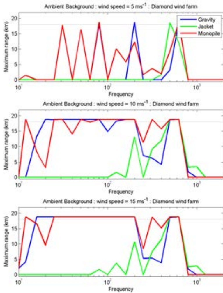
Figure 4-7 – Maximum range from the centre of a diamond shaped wind farm that wind turbines are audible above the background noise as a function of frequency in Hz. Turbines mounted on gravity bases, jackets and monopiles are compared at three different wind speeds. The Wenz curve used for 5 ms -1 , 10 ms -1 and 15 ms -1 relate to sea states 2, 4 and 6 respectively converted to one-third octave levels. The dotted black line represents the boundary of the far-field domain that was modelled; at points where the maximum range is above the dotted line represents maximum range lies outside of the modelled domain.
