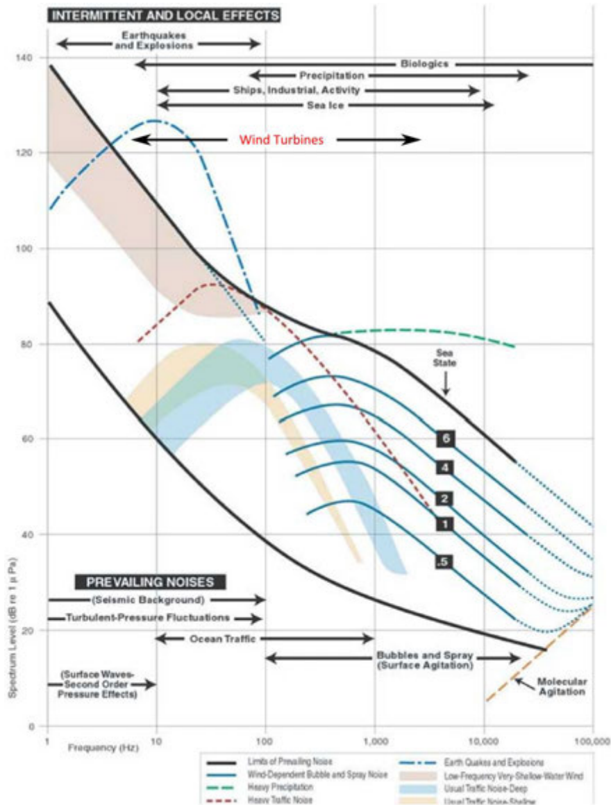
Figure 2-2 Wenz curve showing typical sound levels in the ocean (Wenz 1962) with sound level in units relative to 1 \mu Pa.
