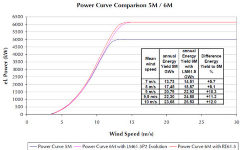
Figure 3-9 Power curve for a REPower 6MW wind turbine, (Doc 9-11). This enables the forces in the gear box and generator to be approximated for different wind speeds.
