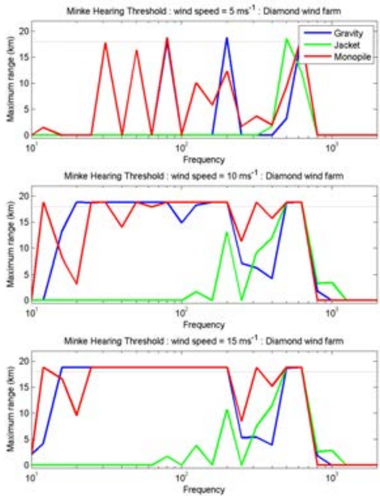
Figure 5-3 - Maximum range at which a minke whale could hear a wind farm at different wind speeds. Gravity base, jacket and monopile foundations are compared. It is assumed that if the SPL is below the background noise that a minke whale could not hear the wind farm. The range is measured to the centre of the wind farm.
