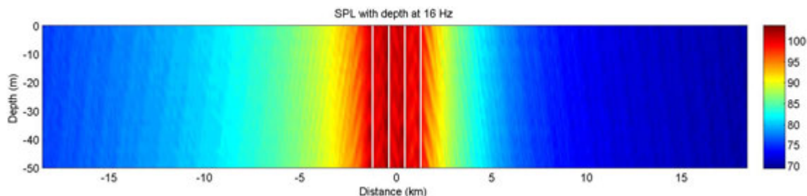
Figure 4-2 – Sound pressure level in a vertical section through an array of 16 wind turbines founded on gravity foundations in a diamond shaped layout. The colour bar represents SPL in dB (re 1 \mu Pa). The vertical white stripes show the positions of wind turbine foundations that the vertical plane intersects. The SPL was modelled for a wind speed of 15 \text{ ms}^{-1} .
