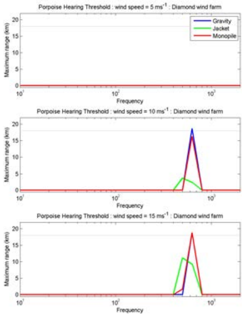
Figure 5-4 - Maximum range at which a porpoise could hear a wind farm at different wind speeds. Gravity base, jacket and monopile foundations are compared. It is assumed that if the SPL is below the background noise that a porpoise could not hear the wind farm. The range is measured to the centre of the wind farm.
