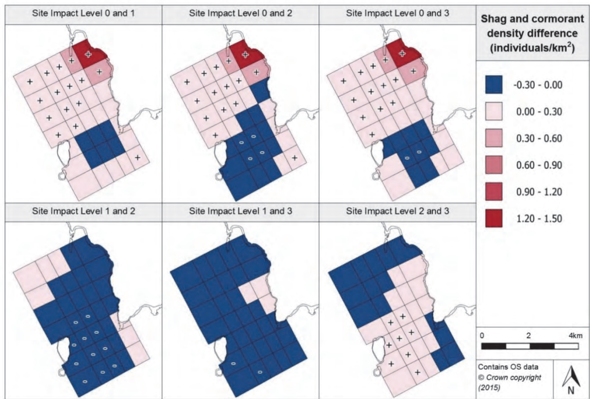
Figure 4.3.27. Estimated density difference between various site impact levels for shags and cormorants during 2011 (year with least variation)
