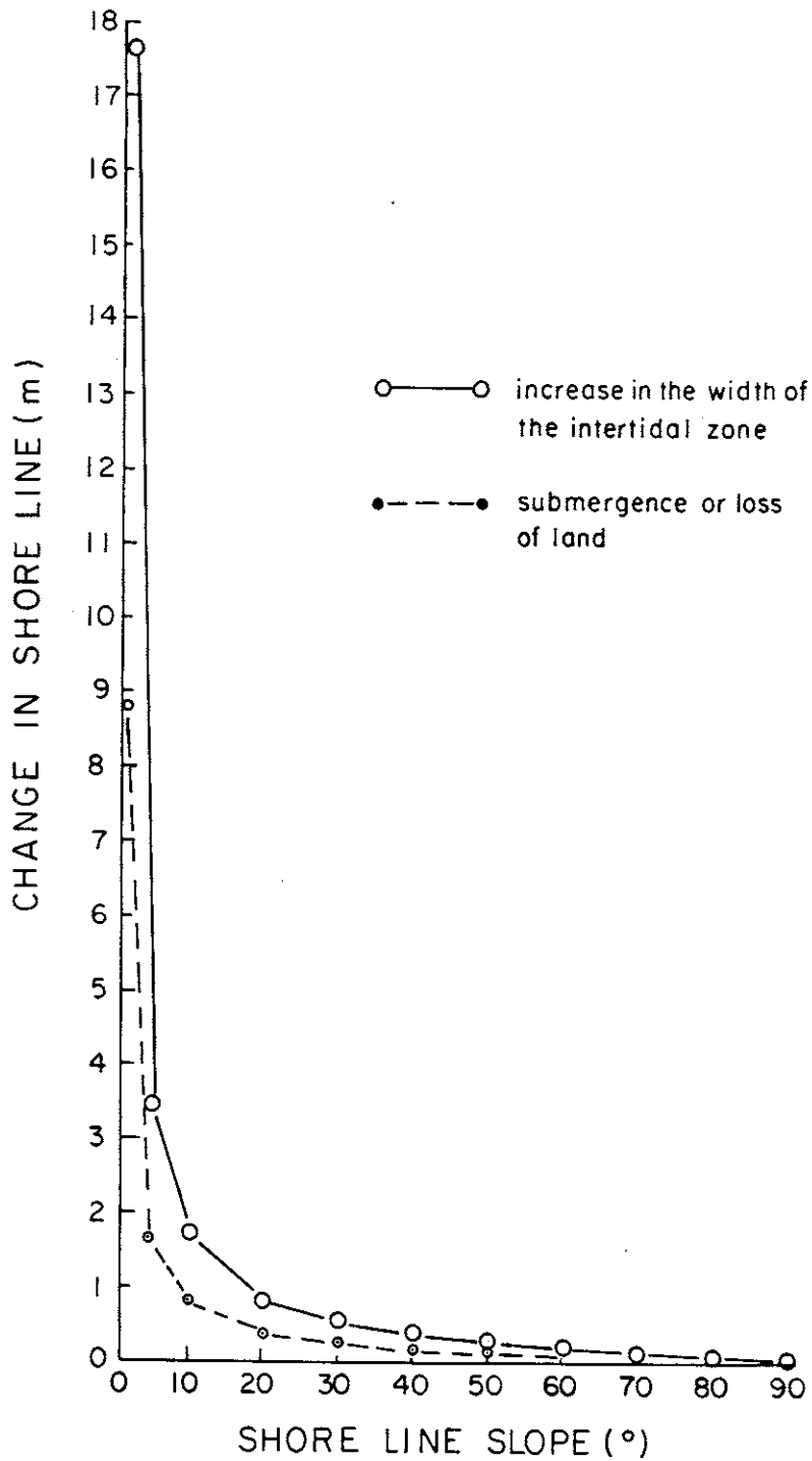
Fig. 4. The influence of shoreline slope and a predicted 30 cm increase in tidal range on the creation of intertidal area and the loss of land.
