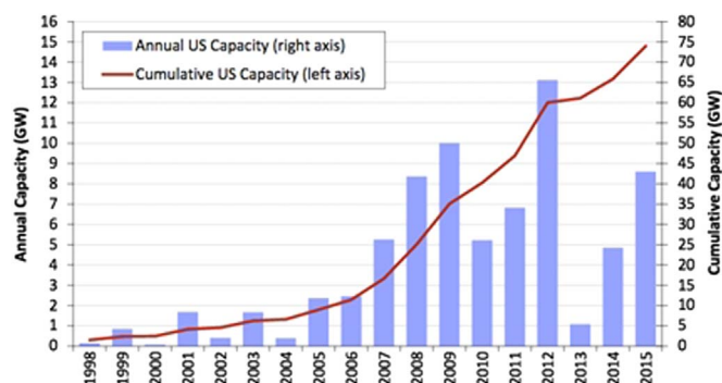
Fig. 3. Annual and cumulative capacity in U.S. wind power capacity [27]. Ref: [29] Wisner, R. & M. Bolinger, 2016. 2015 Wind Technologies Market Report. Lawrence Berkeley National Laboratory (LBNL), Berkeley.
