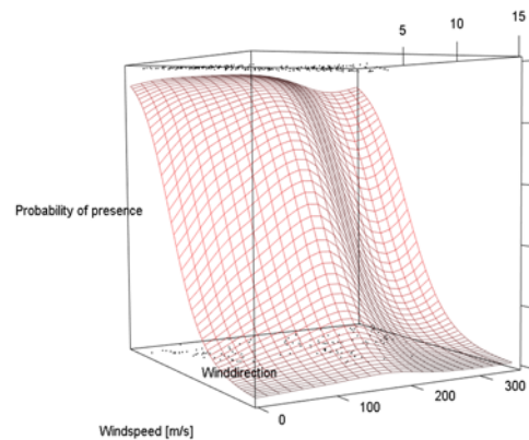
Figure 3.61 Probability of presence LM as a function of the covariates wind speed and wind direction.
