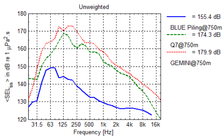
Fig. 9. Draining of seawater from BLUE 25M hammer upon completion of piling operation (left). Frequency spectrum of BLUE piling compared to impact piling at two reference piles (right, note different dimensions: BLUE Piling test: \varnothing 6.5 m, water depth 22 m; reference Gemini OWF: \varnothing 6.6 m, water depth 30 m; reference Q7 OWF: \varnothing 4 m, water depth 19-24 m), © Fistuca BV.
