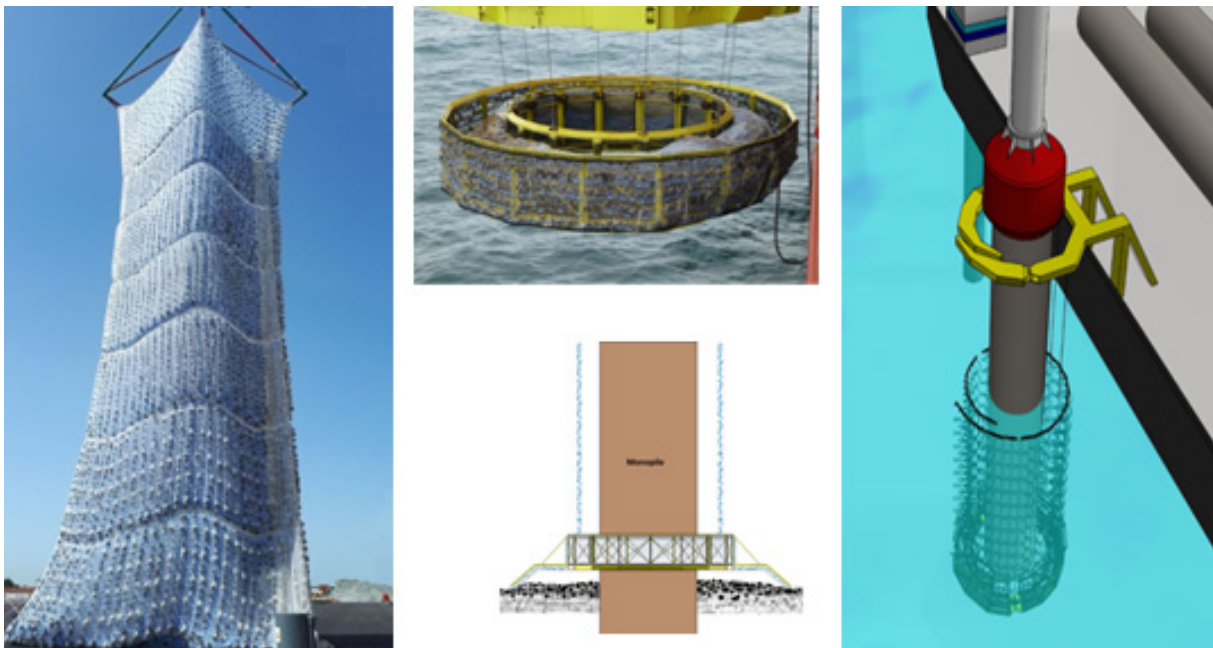
Fig. 4. HSD net for a water depth of 40 m with larger HSD elements on the bottom (due to compressibility with hydrostatic pressure (left). HSD basket below pile frame (center, top). Concept of a HSD basket covering the sea floor close to the pile in order to mitigate also ground coupling effects (center, bottom). Concept of an openable HSD basket for very long monopiles to be inserted sideways (right). © K.-H. Elmer, OffNoise Solutions.
