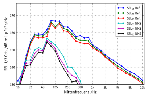
Fig. 3. Monopile installation at the OWF Borkum Riffgrund 1 using the Integrated Monopile Installer with NMS (left, © Ørsted). Frequency spectra (SEL third-octave band level) of ramming noise with and without NMS at OWF Borkum Riffgrund 1, measured 750 m from the pile given as percentiles (right, Gündert et al. 2015).
