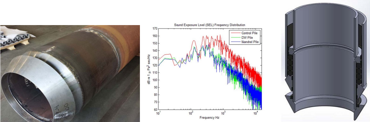
Fig. 7. Double pile stem with driving shoe (left), SEL frequency distribution (middle) during piling of control pile (red) and double pile configurations (green and blue), ( Reinhall et al., 2015). Schematic of flexible coupling to connect outer and inner pile in the driving shoe (right, Reinhall et al., 2016).
