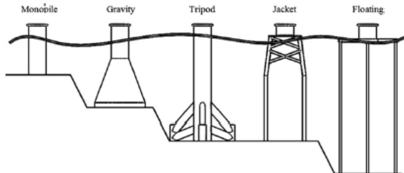
Figure 3-1. Some of the offshore wind turbine foundation types. Taken from Higgins & Foley, 2014.
