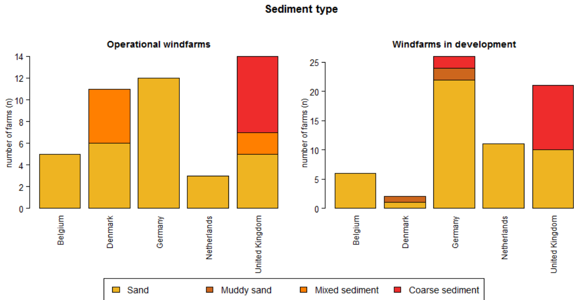
Figure 4-2. Graph on the left; seabed sediment type of operational wind farms at the time of writing of this report. Graph on the right; seabed sediment types of wind farms that are currently in development.
