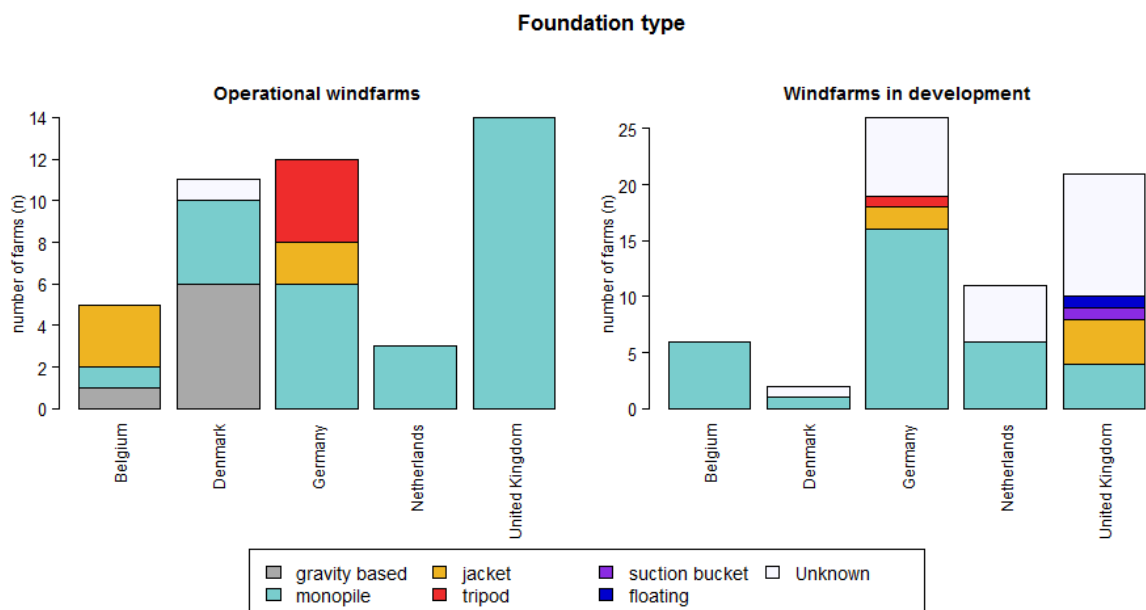
Figure 4-3. Graph on the left; foundation types of fully operational wind farms at the time of writing of this report. Graph on the right; foundation types of wind farms that are currently in development.
