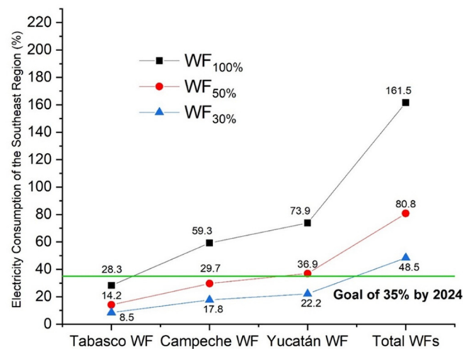
Figure 10. Contribution of wind farms to electricity consumption in the Southeast Region under three installed capacity scenarios.
