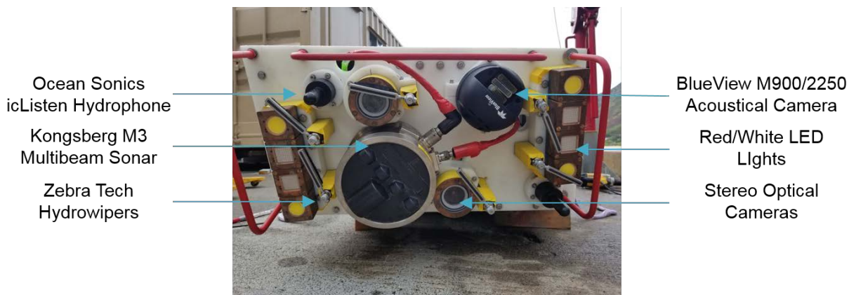
Fig. 3. WAMP instrument head.
