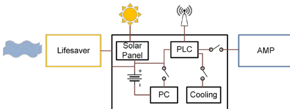
Fig. 5. Block diagram of WAMP control box components.
