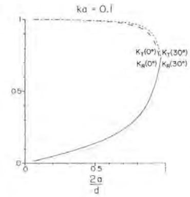
FIGURE 2. COEFFICIENTS OF REFLECTION AND TRANSMISSION FOR WAVE SCATTERING BY A ROW OF CIRCULAR CYLIDERS ( KA = 0.1 ) (From R.A. Dalrymple et al.,1988)
