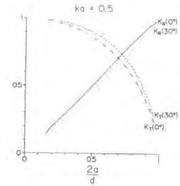
FIGURE 3. COEFFICIENTS OF REFLECTION AND TRANSMISSION FOR WAVE SCATTERING BY A ROW OF CIRCULAR CYLIDERS ( KA = 0.5 ) (From R.A. Dalrymple et al.,1988)
