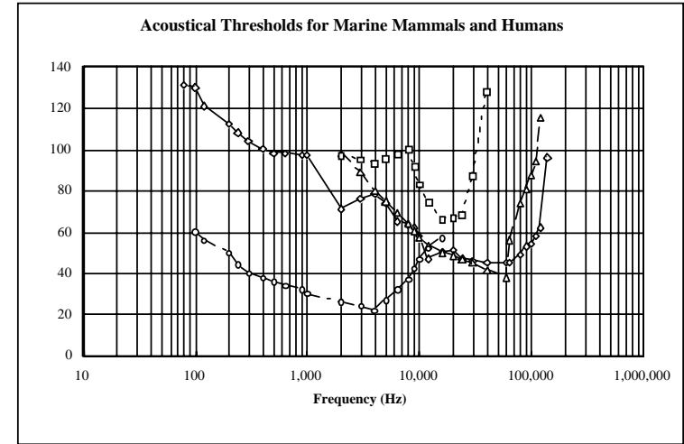
Figure 7-3 Acoustic Thresholds of Two Porpoises and the Hawaiian Monk Seal in Water, and Humans in Air
