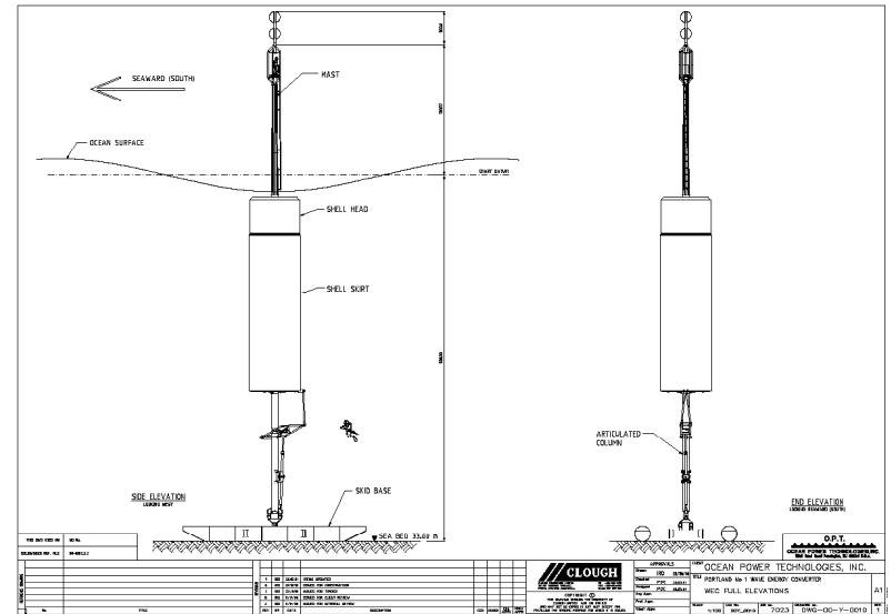
Figure 5-1 Wave Energy Technology Offshore Components
