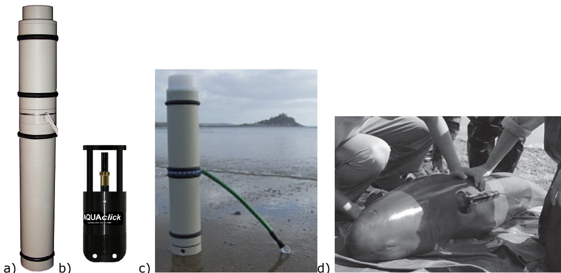
Figure 6-9: Different passive acoustic devices: a) T-POD 1 , b) AquaClick 100 (PCL) 2 c) C-POD 1 d) A-Tag, attached with suction cups to a finless porpoise (from Akamatsu et al. 2005)
