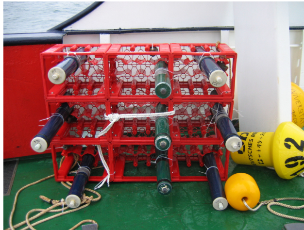
Figure 6-12: Intracalibration of T-PODs close to the wind farm Nysted, from Verfuß et al. (2007c), the devices are separated by at least 30 cm to prevent a bias from interferences and echoes.
