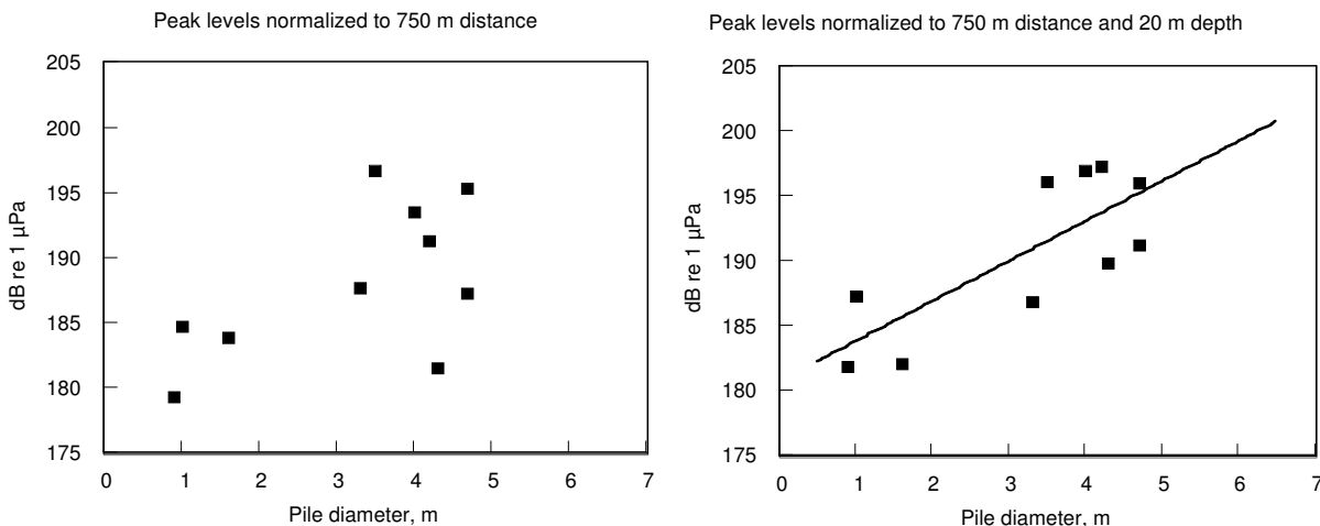
Figure 2-1: Peak levels of pile driving blows versus pile diameter. Left: Normalised to equal distance only. Right: With additional normalisation to 20 m water depth. The regression line in the right diagram has a slope of 3.1 D , where D is the pile diameter in metres (from Nehls et al. 2008).
