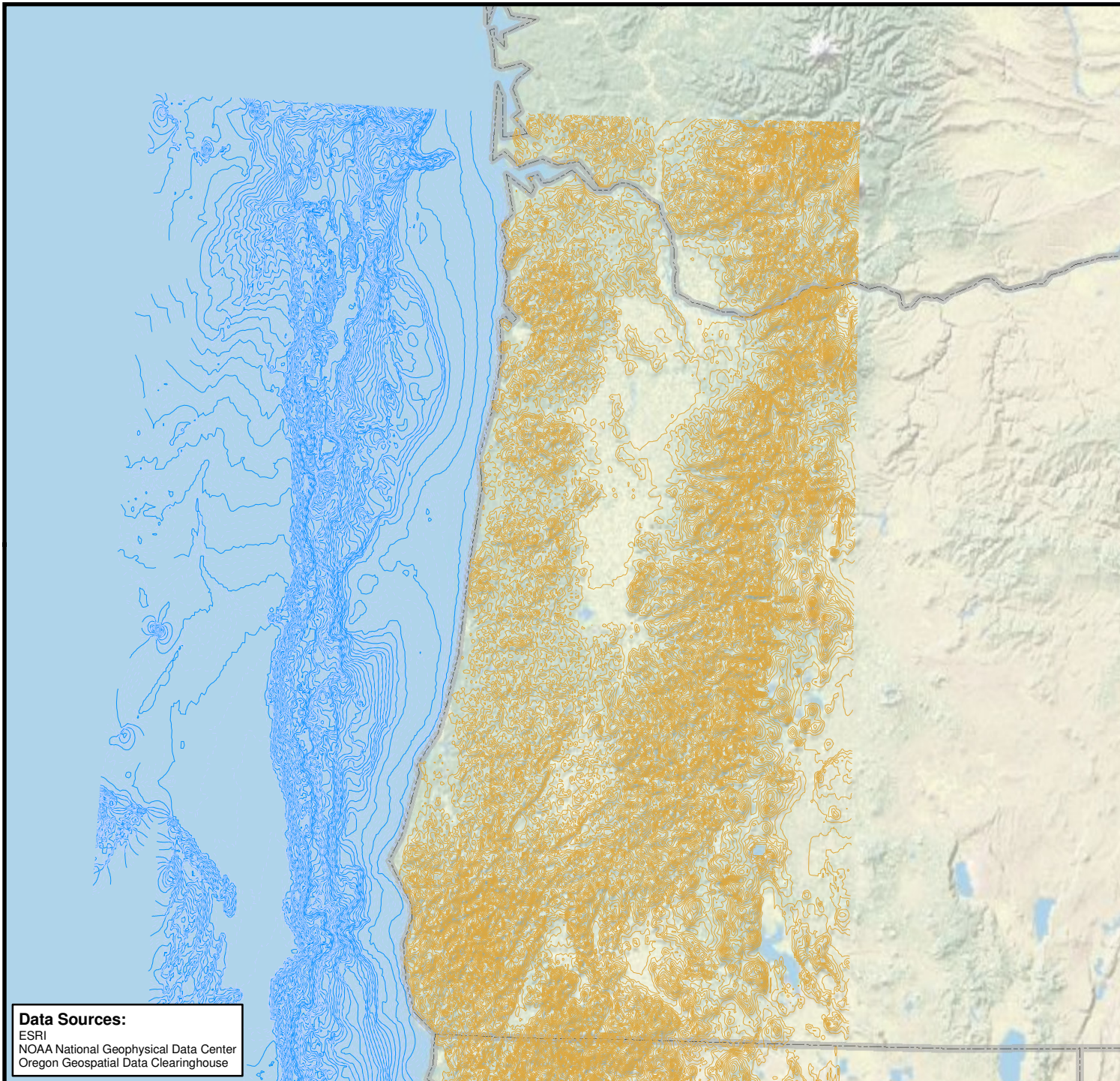
Fig. 1-1 Bathymetry
