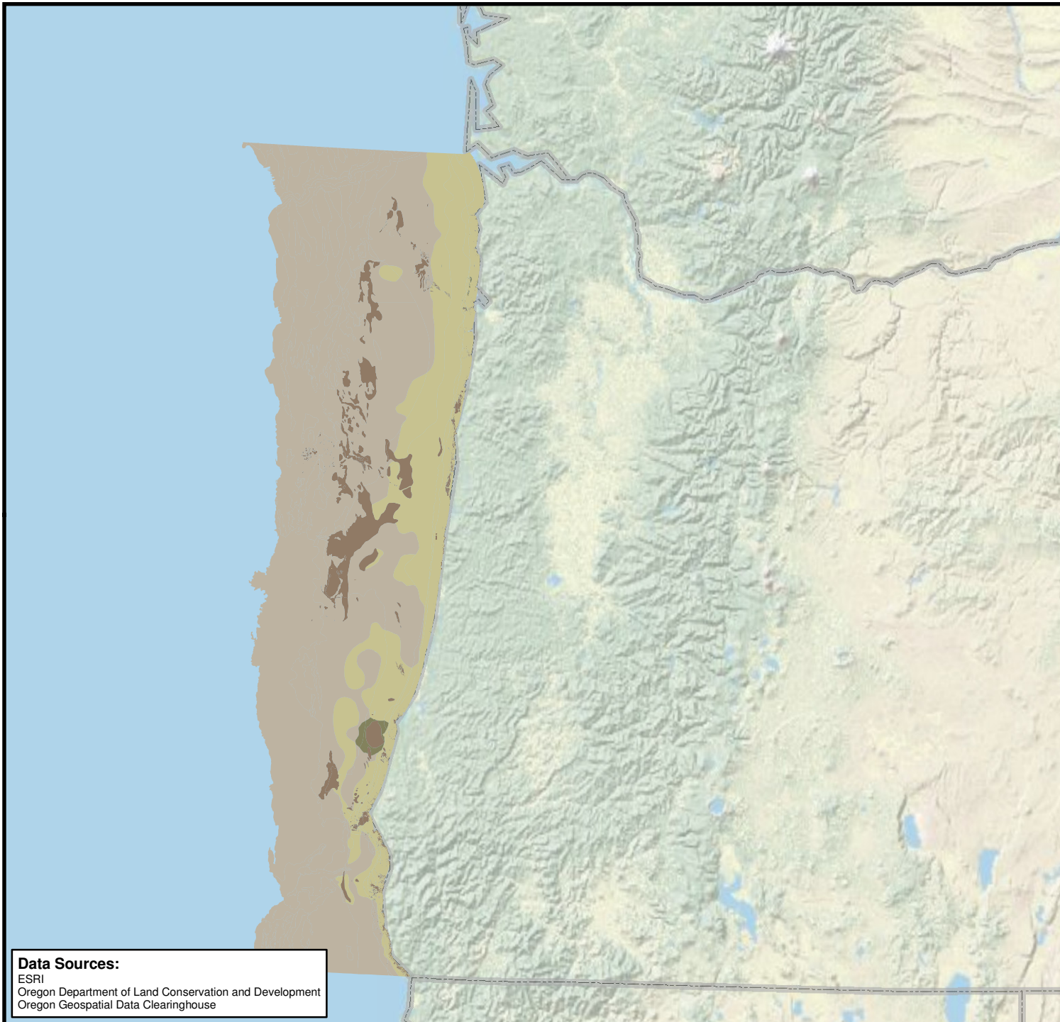
Fig. 1-2 Seabed Type
