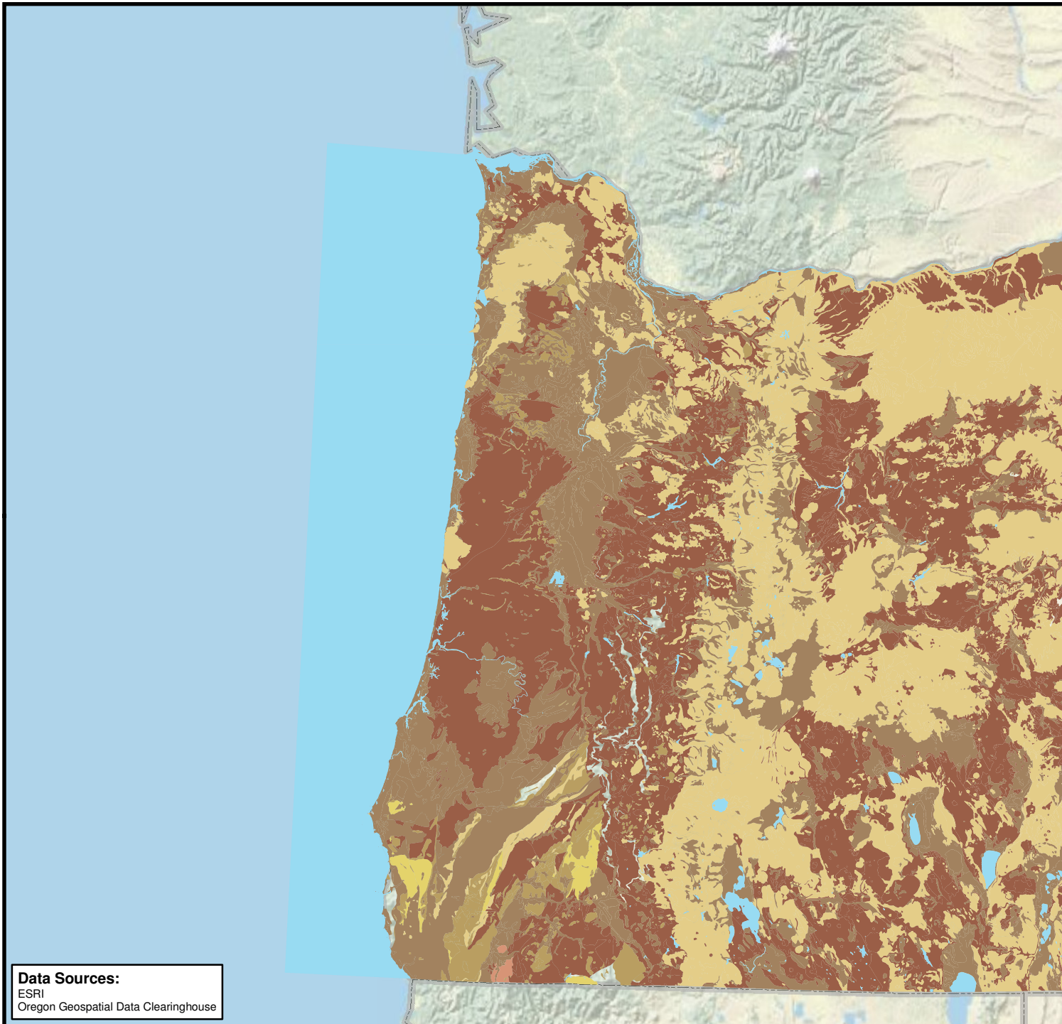
Fig. 1-4 Geology
