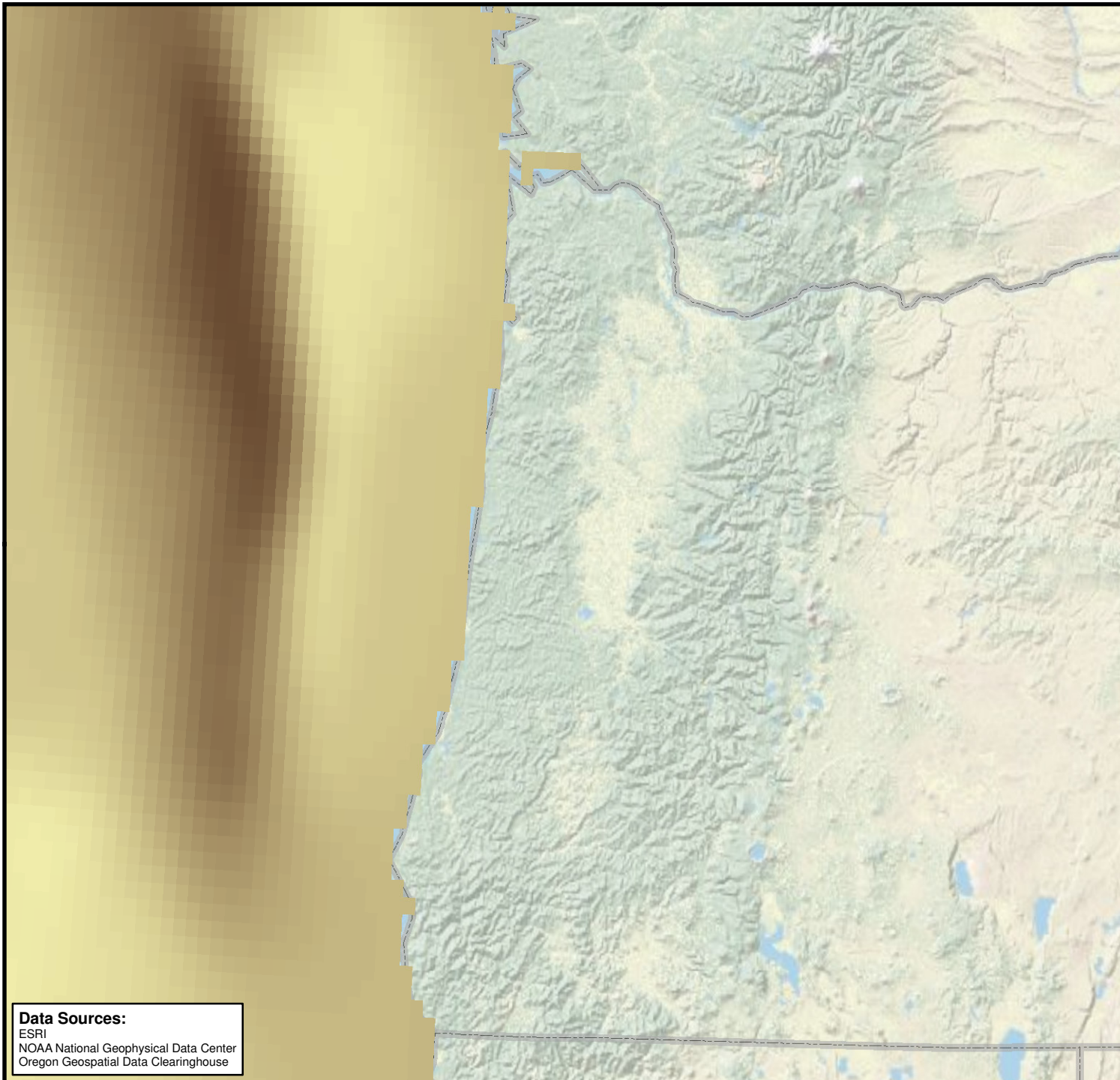
Fig. 1-3 Sediment Depth
