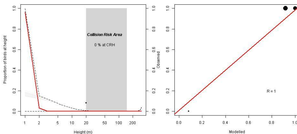
Figure 3.22 Little Auks (Left) Median modelled height distribution based on boat-based survey data (red line), height distribution based on each bootstrap also shown (grey lines), plotted with raw data showing the proportion of birds in each height band. (Right) Modelled vs observed proportions of birds in each height band. (Circle diameter is proportional to the square root of the number of birds recorded in each band).
