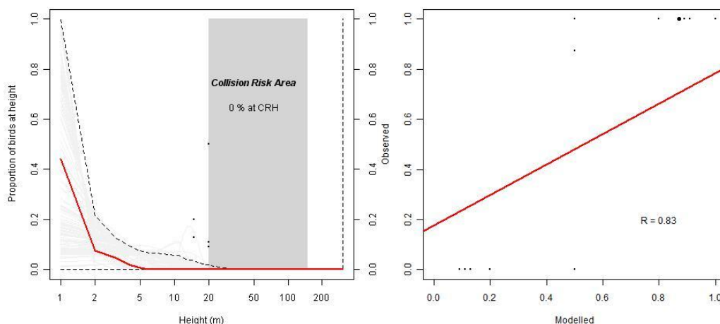
Figure 3.3 Black-throated Diver (Left) Median modelled height distribution based on boat-based survey data (red line), height distribution based on each bootstrap also shown (grey lines), plotted with raw data showing the proportion of birds in each height band. (Right) Modelled vs observed proportions of birds in each height band. (Circle diameter is proportional to the square root of the number of birds recorded in each band).
