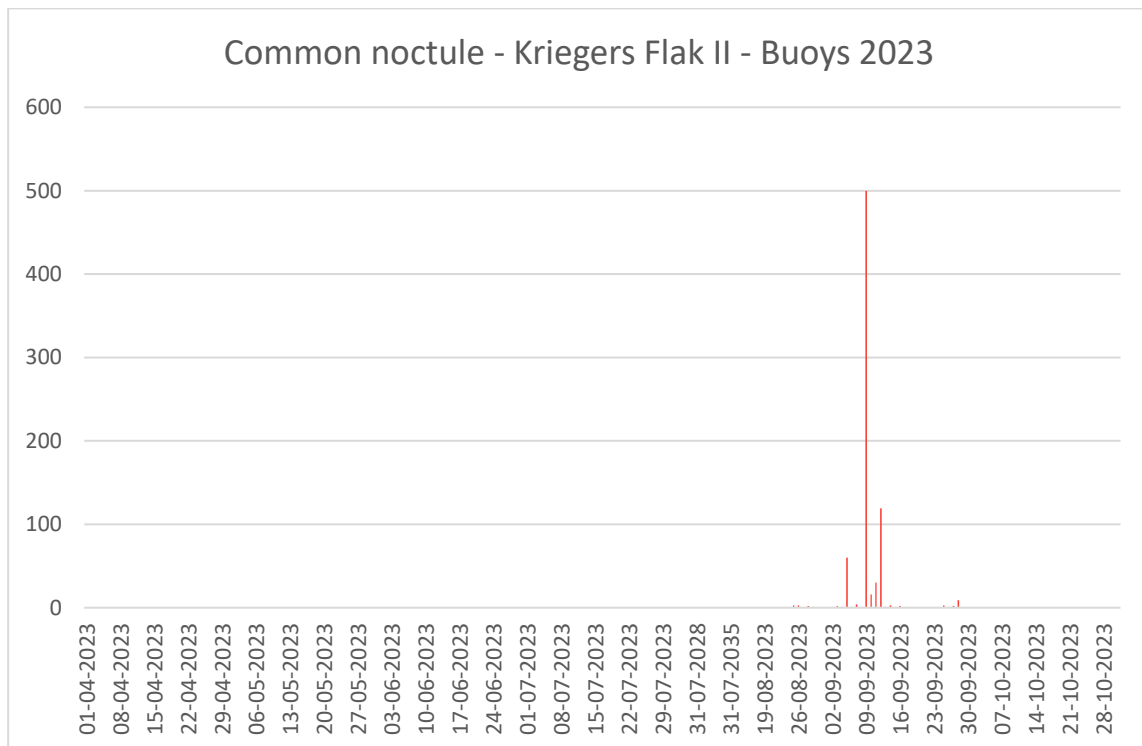
Figure 14 - Total number of common noctule recordings (from 16 buoys) per night in 2023.
