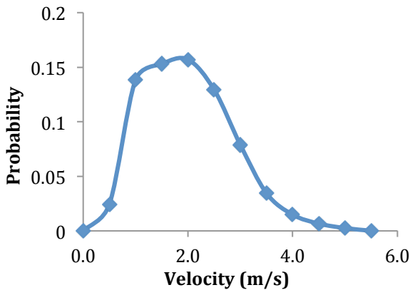
Fig. 5 Probability distribution for velocity at the location of impact between the whale and blade.
