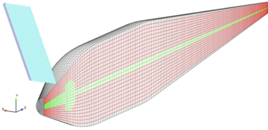
Fig. 4 Finite element analysis model setup of whale (in red and green) and single blunt edge turbine blade (in blue).
