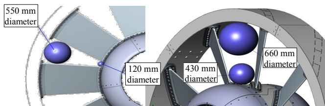
Fig. 3 Drawings of the OpenHydro turbine blade assembly, as specified by OpenHydro, showing spacing of blade edges (left) and the spacing between blades (right). The details of the design were used in the engineering analysis.
