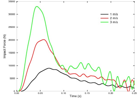
Fig. 6 Impact force as a function of time for different blade speeds
