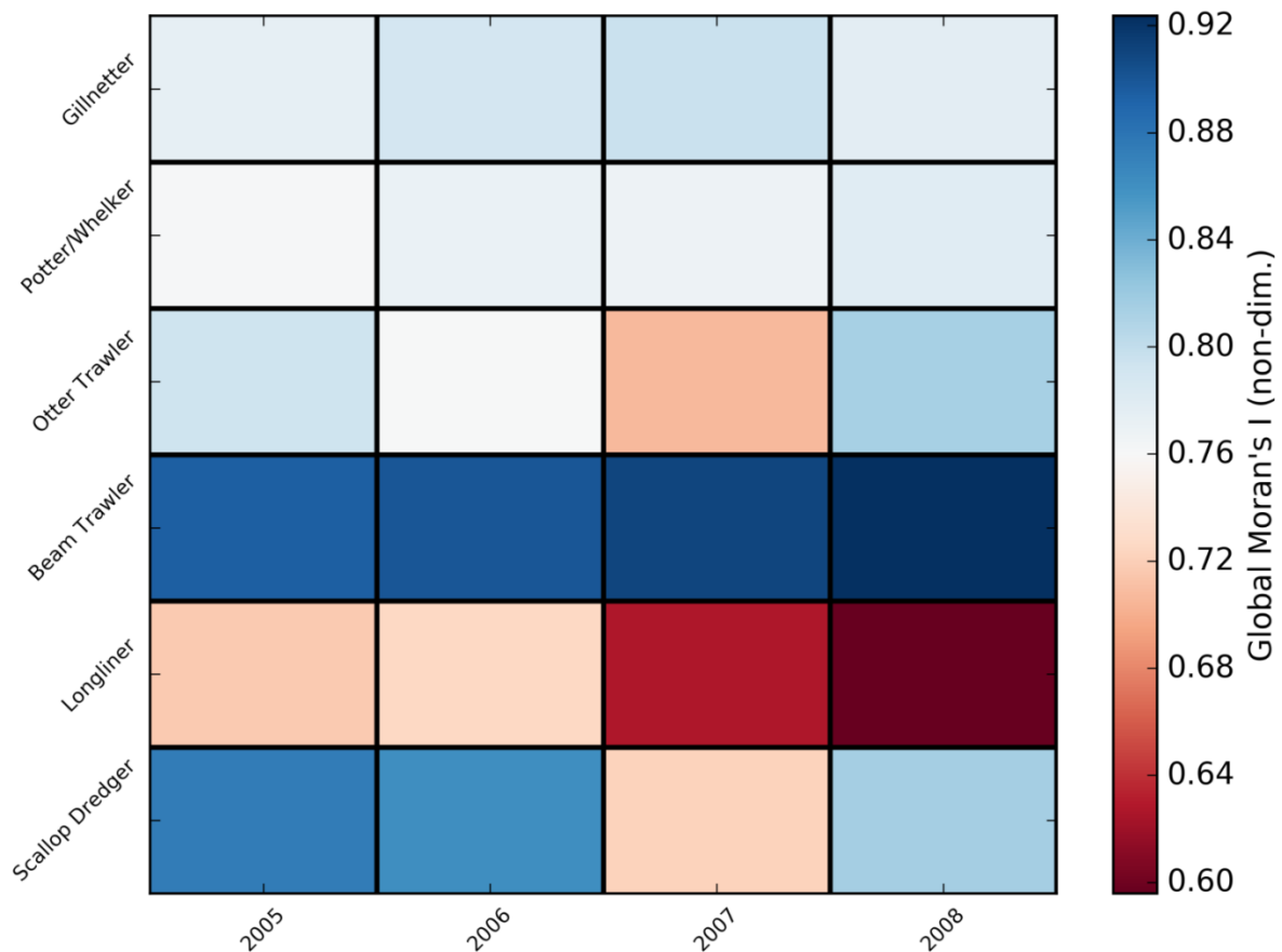
Figure 3.10 Global Moran's I
