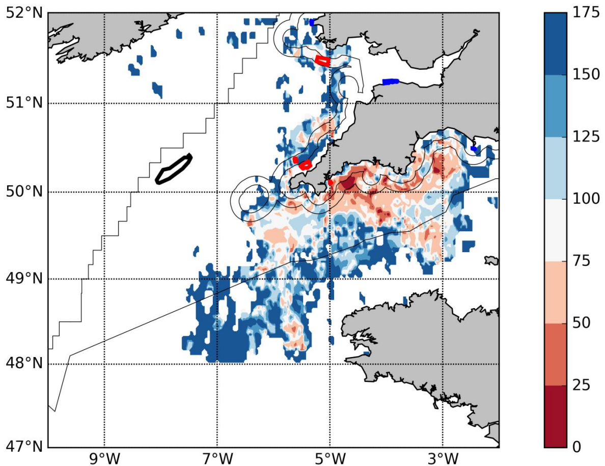
Figure 4.16 Coefficient of Variation (CV) of longliner fishing effort per grid cell Coefficient of variation of longliner fishing effort expressed as a percentage of the mean fishing effort per grid cell, over 2005-2008. Haig Fras (black polygon) and MREIs (red/blue polygons) are marked.
