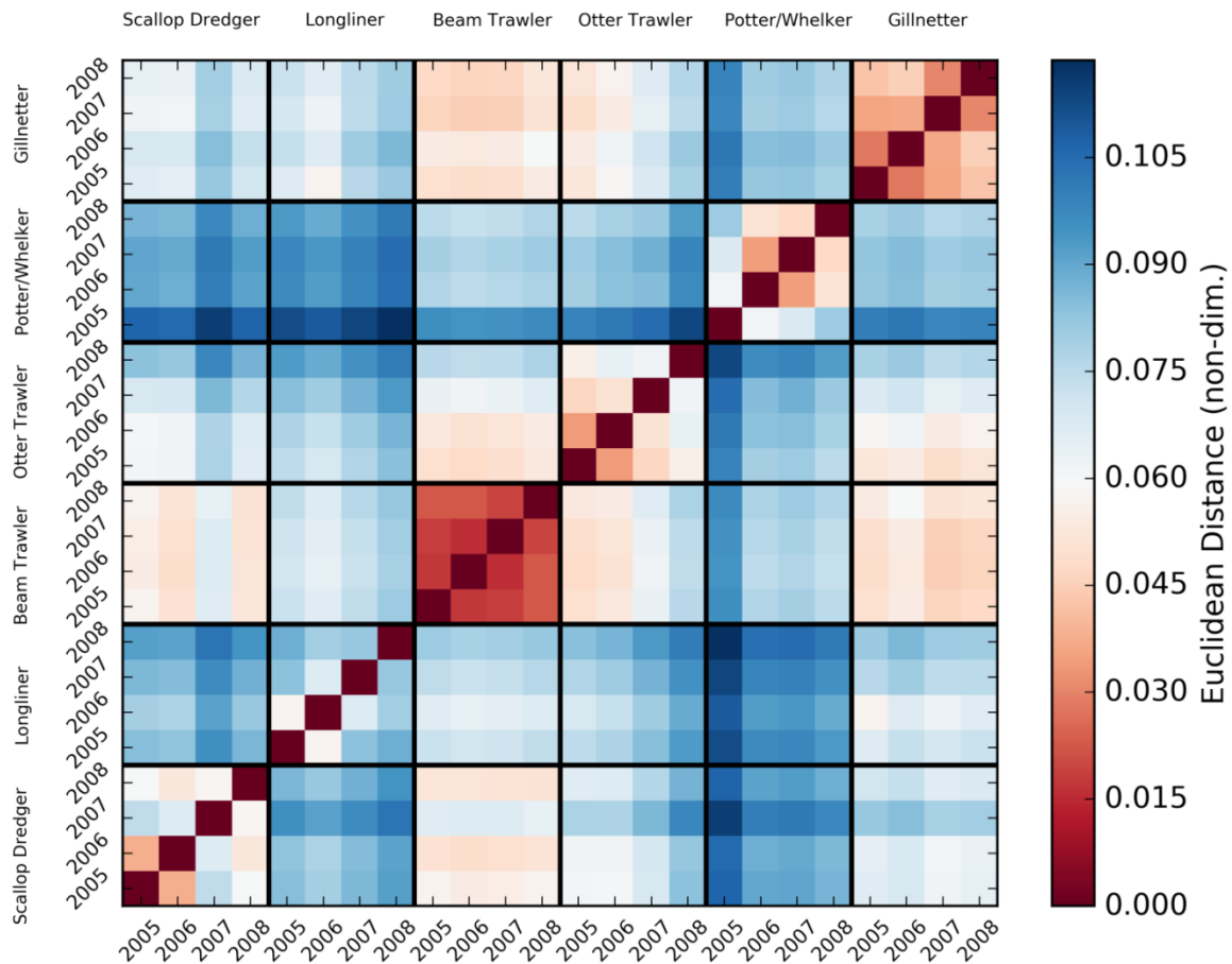
Figure 3.3 The Euclidean distance matrix between all gears and all years.
