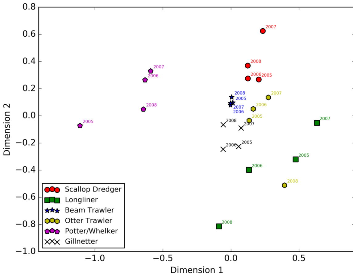
Figure 3.2 2-D MDS ordination of fishing activity of scallop dredgers, longliners, beam trawlers, otter trawlers, potter/whelkers and gillnetters between gears and between years.
