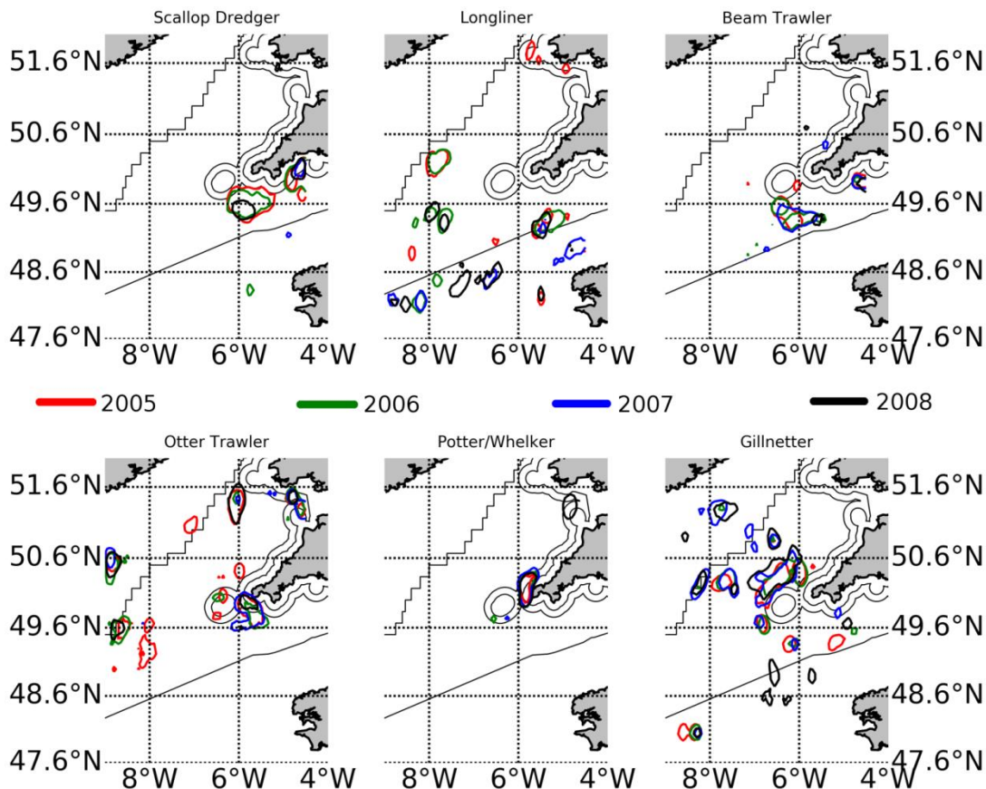
Figure 3.11 Getis-Ord Gi Statistic for all gear-types between 2005-2008.
