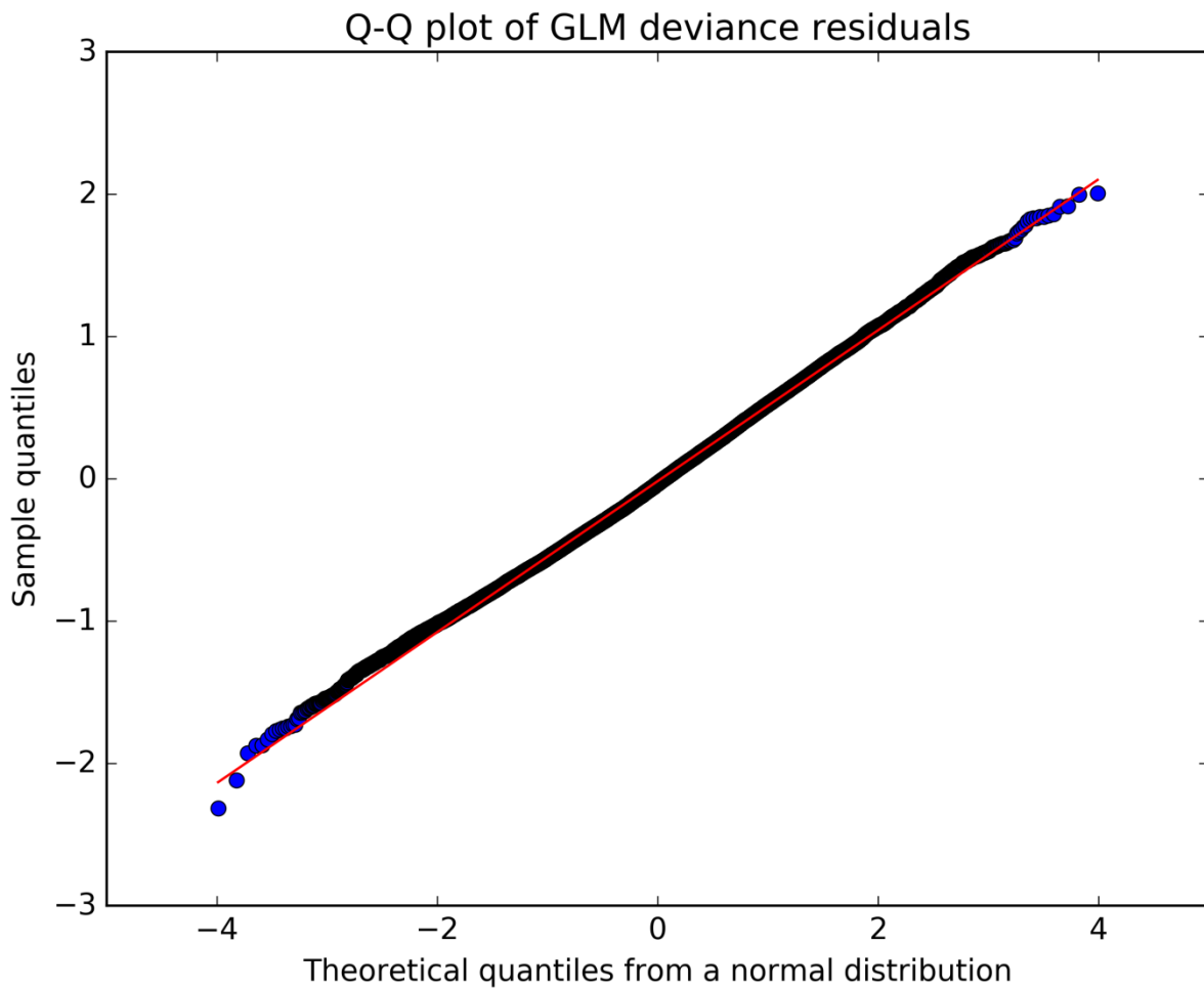
Figure 4.12 Quantile-Quantile plot of the residuals in the model
