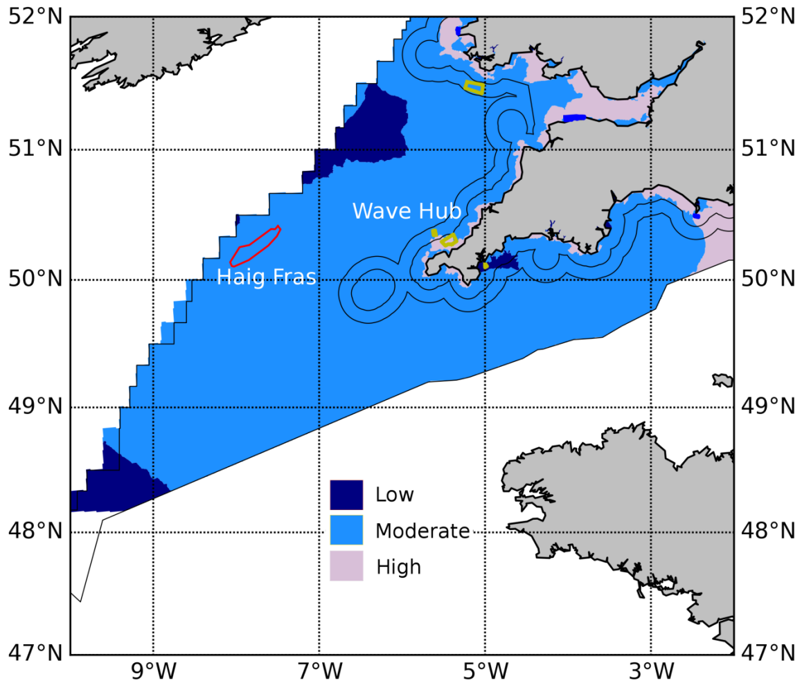
Figure 4.1: Kinetic energy at the seabed in the South West UK waters
