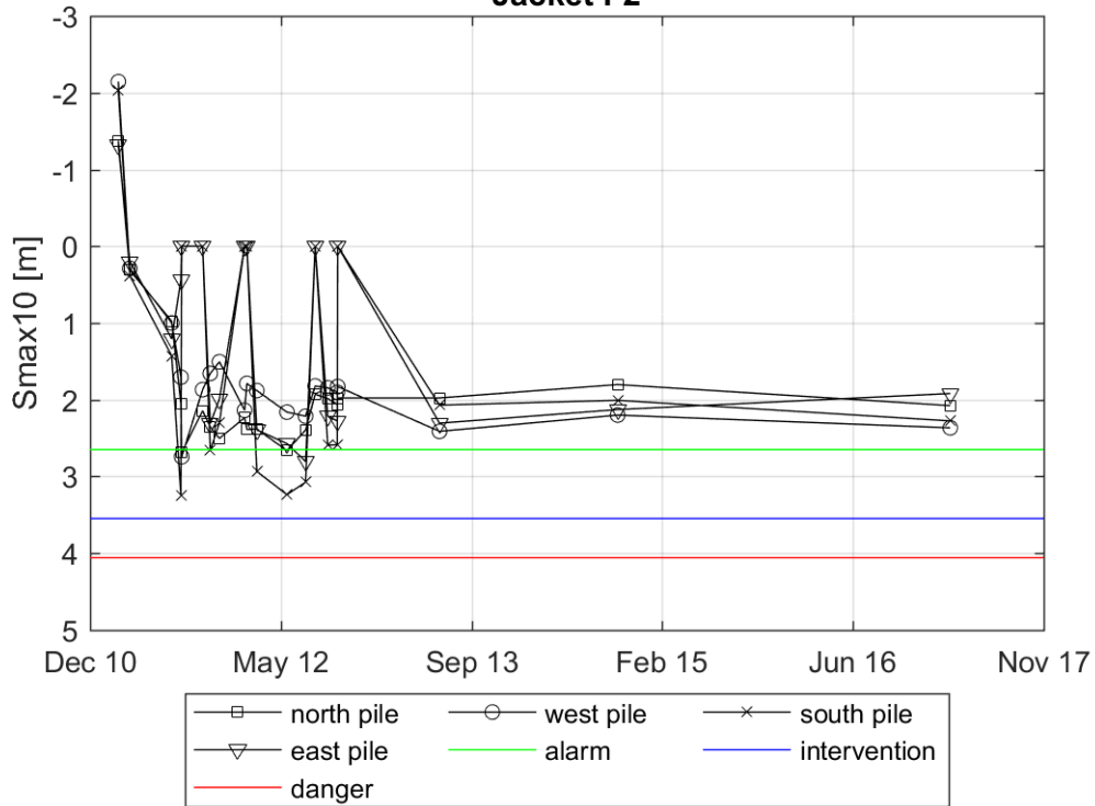
Evolution of Smax10 in a radius of 3m around the pile Jacket F2
