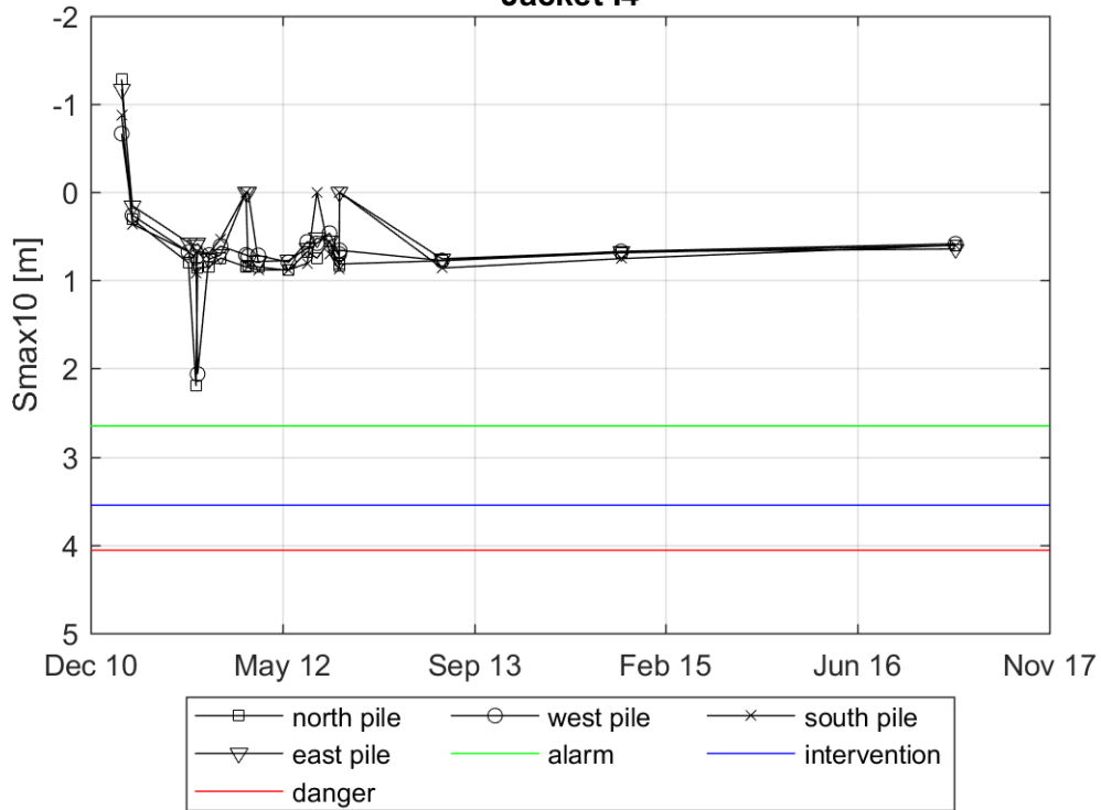
Evolution of Smax10 in a radius of 3m around the pile Jacket I4
