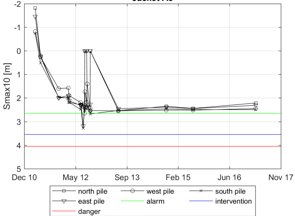
Evolution of Smax10 in a radius of 3m around the pile Jacket A5
