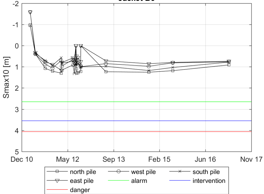
Evolution of Smax10 in a radius of 3m around the pile Jacket B6
