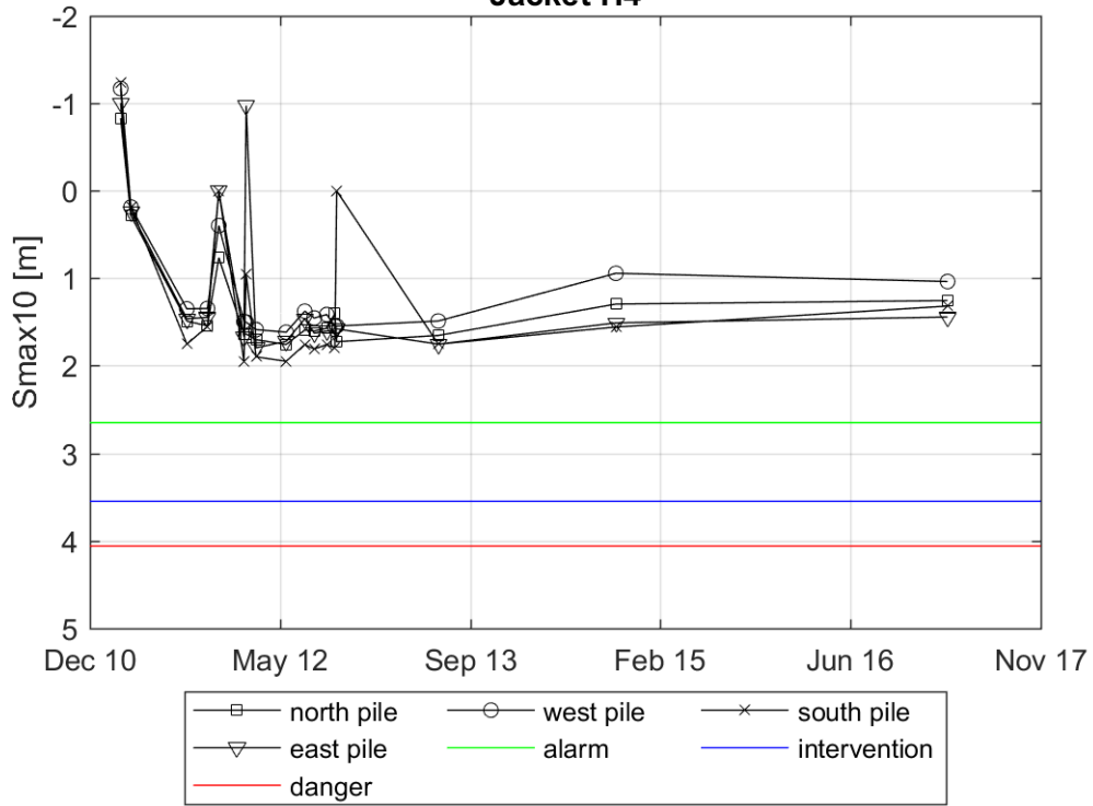
Evolution of Smax10 in a radius of 3m around the pile Jacket H4
