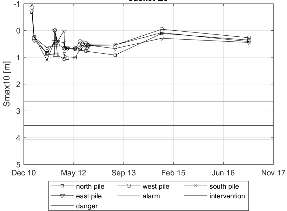
Evolution of Smax10 in a radius of 3m around the pile Jacket E5
