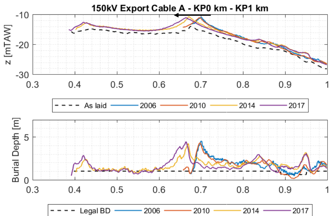
Figure 4-1: Detail of the Depth of Cover along export cable A, zone A1
