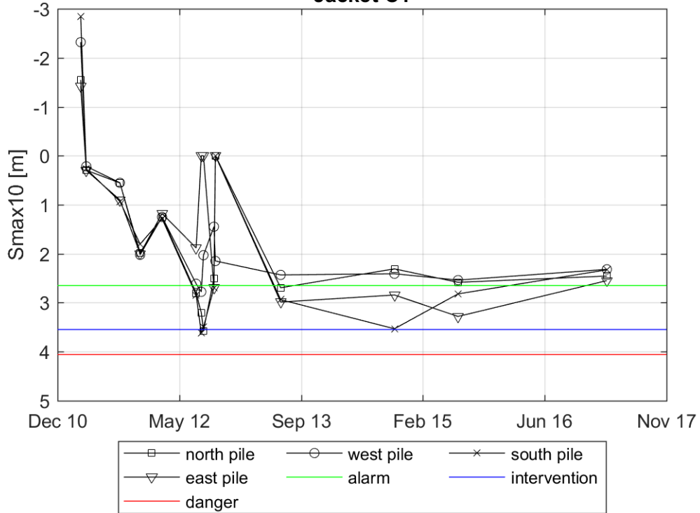
Evolution of Smax10 in a radius of 3m around the pile Jacket C1
