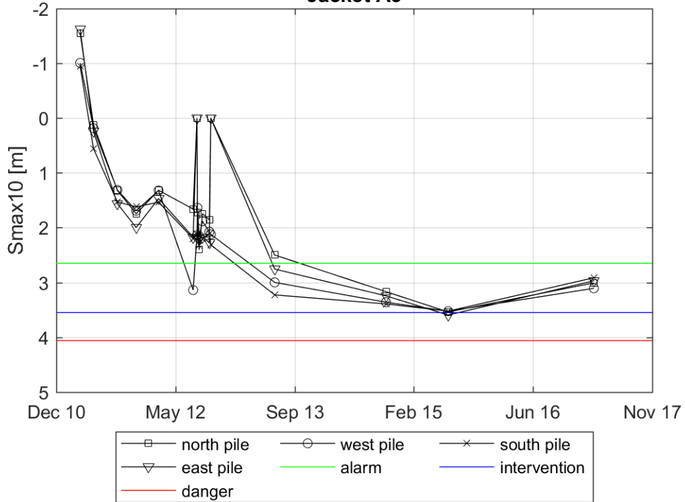
Evolution of Smax10 in a radius of 3m around the pile Jacket A3
