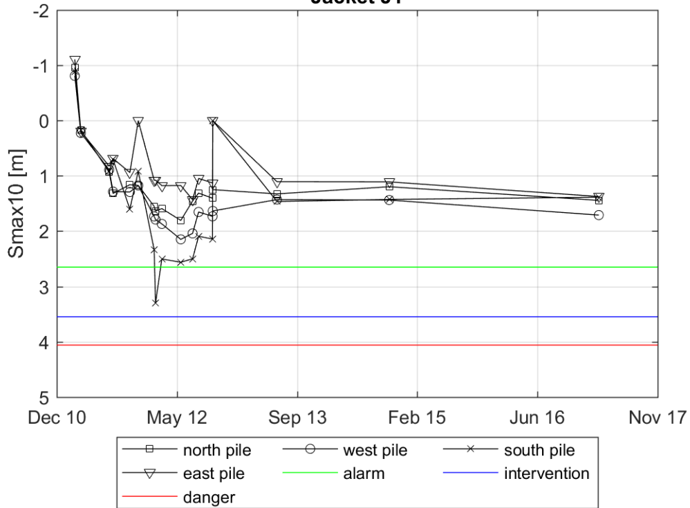
Evolution of Smax10 in a radius of 3m around the pile Jacket J1
