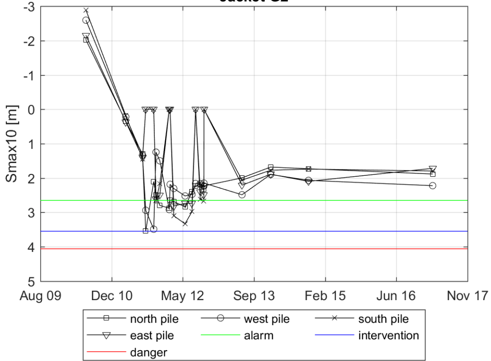
Evolution of Smax10 in a radius of 3m around the pile Jacket G2
