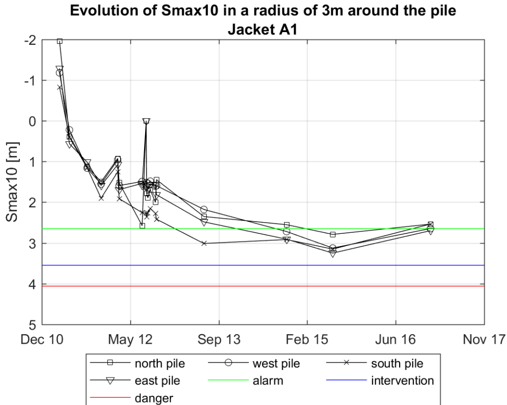
Figure 3-1: Evolution of the scour depth ( S_{max10} ) around the piles of Jacket foundation A1.
