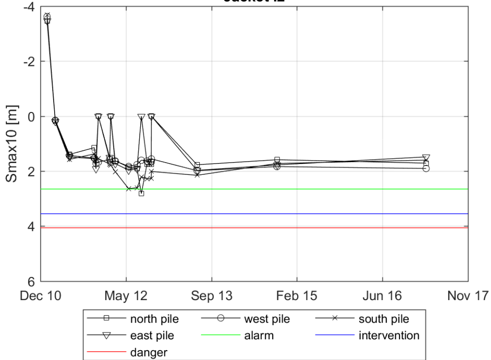
Evolution of Smax10 in a radius of 3m around the pile Jacket I2
