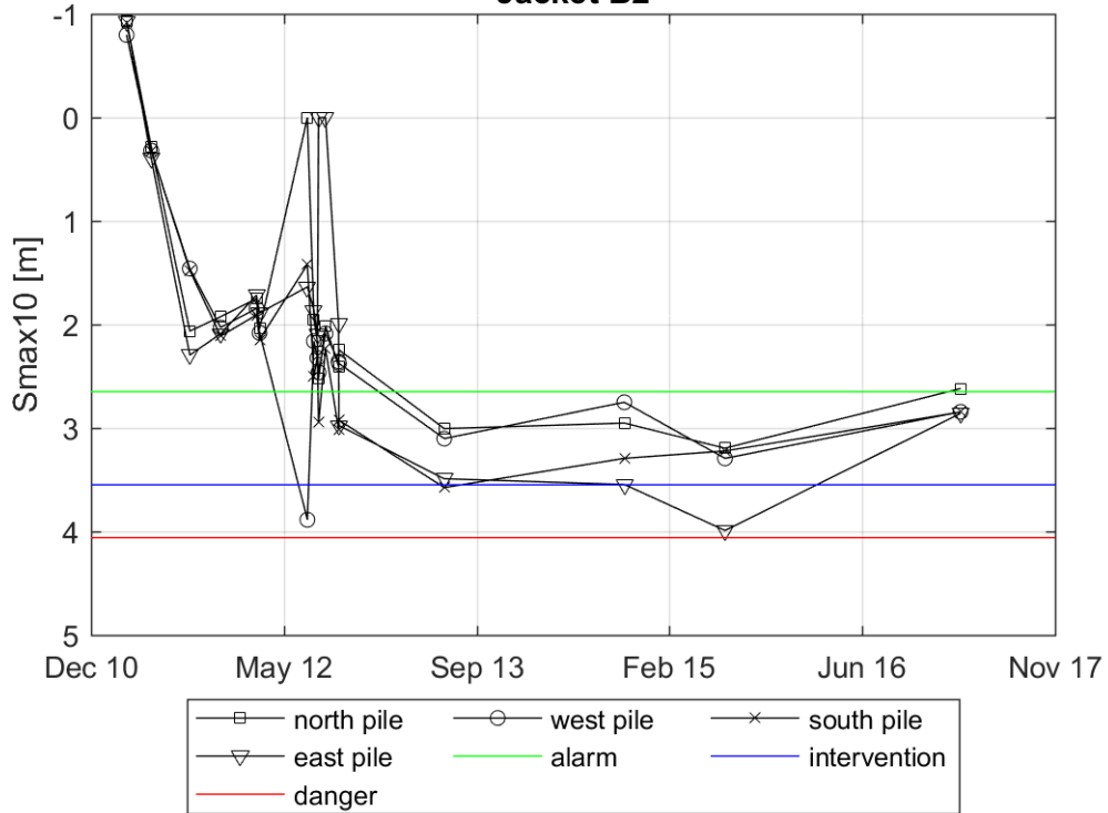
Evolution of Smax10 in a radius of 3m around the pile Jacket B2
