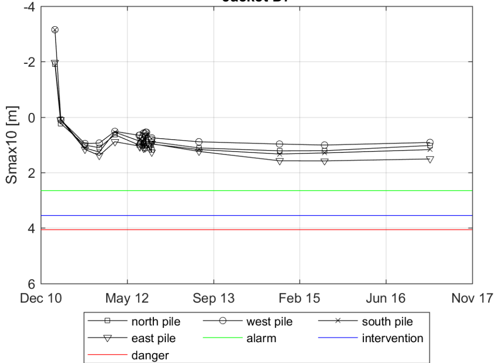
Evolution of Smax10 in a radius of 3m around the pile Jacket D7
