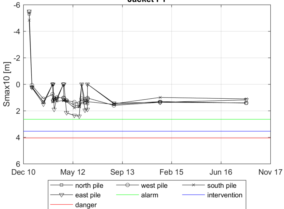
Evolution of Smax10 in a radius of 3m around the pile Jacket F1
