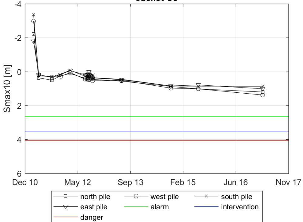
Evolution of Smax10 in a radius of 3m around the pile Jacket C5
