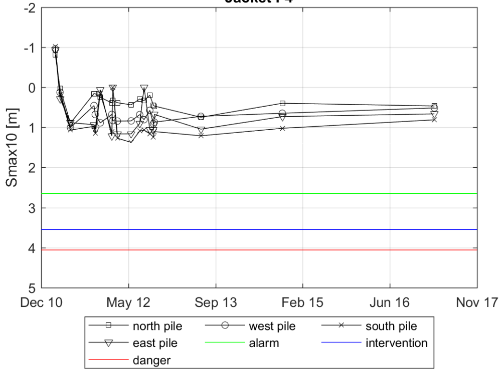
Evolution of Smax10 in a radius of 3m around the pile Jacket F4
