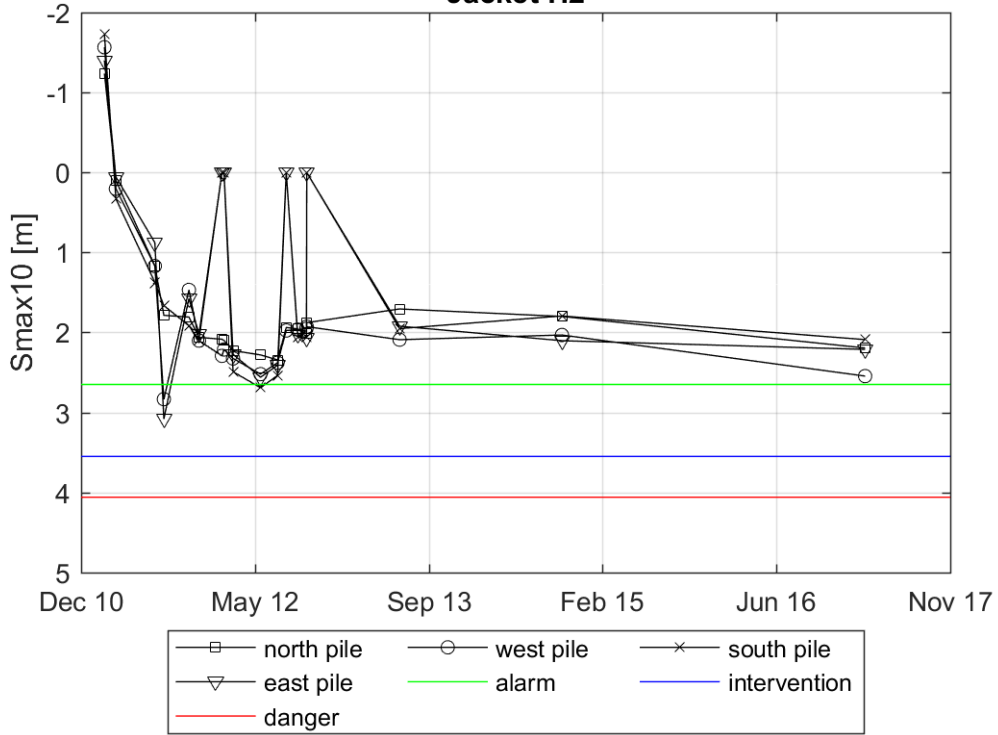
Evolution of Smax10 in a radius of 3m around the pile Jacket H2
