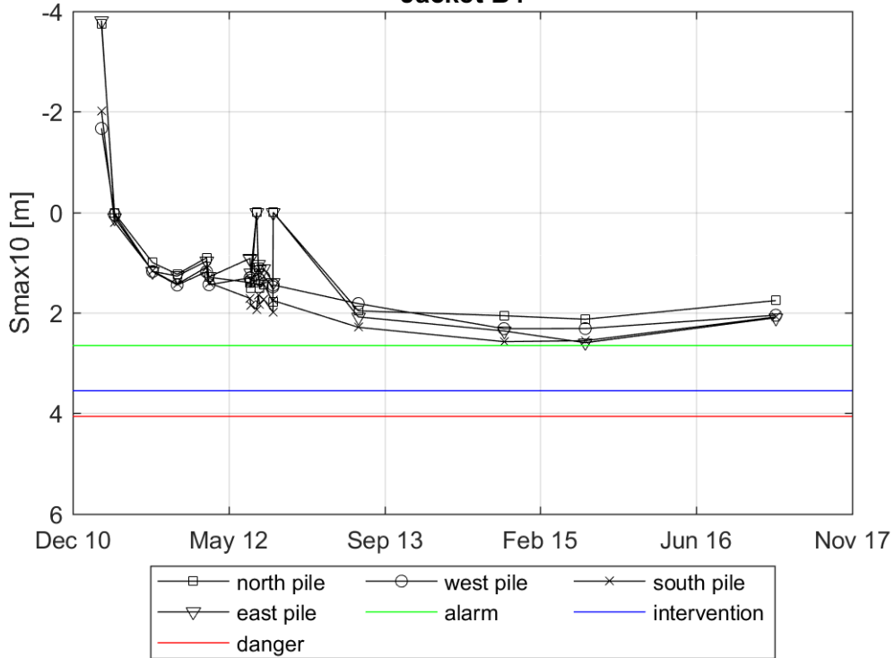
Evolution of Smax10 in a radius of 3m around the pile Jacket B4
