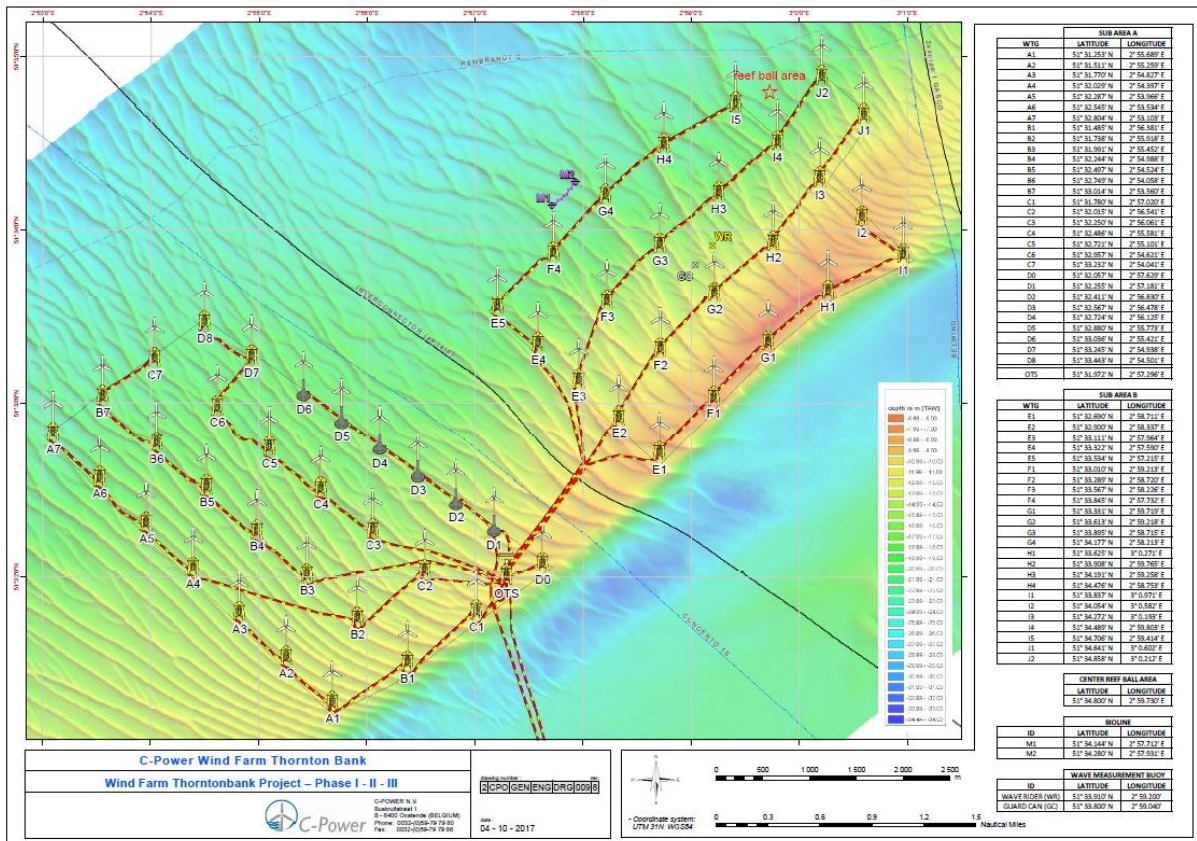
Figure 1: Lay-out of C-Power’s wind farm
