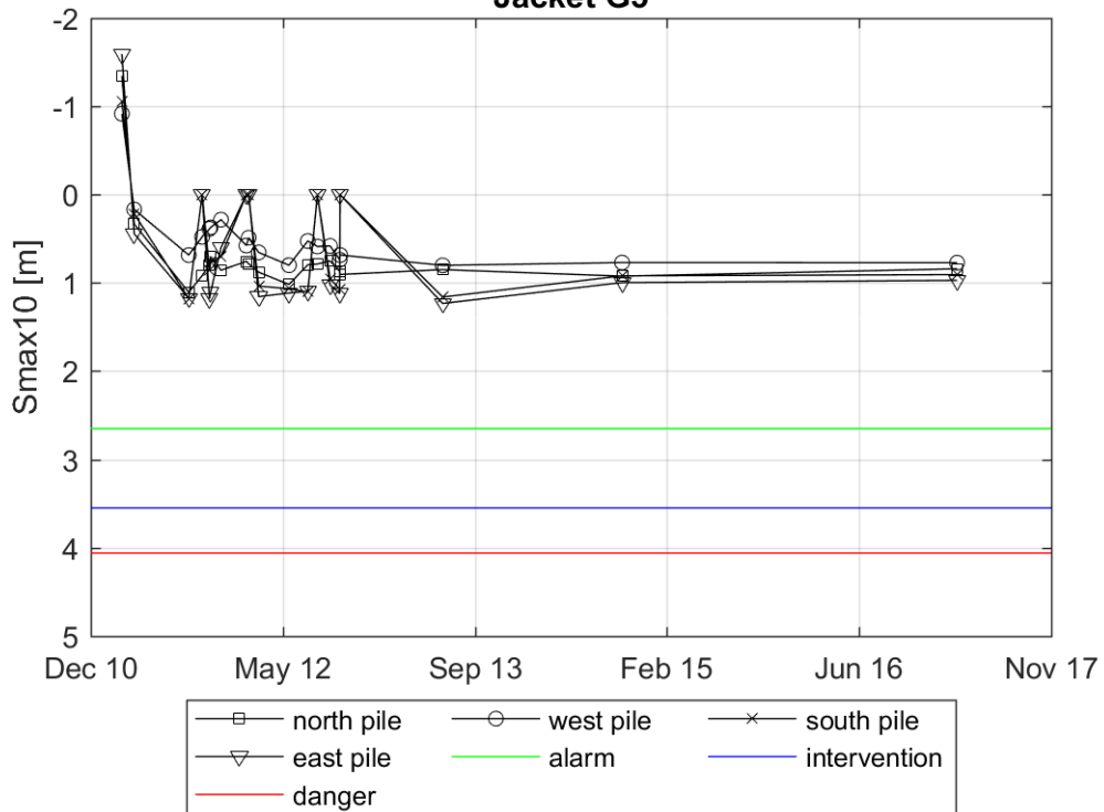
Evolution of Smax10 in a radius of 3m around the pile Jacket G3
