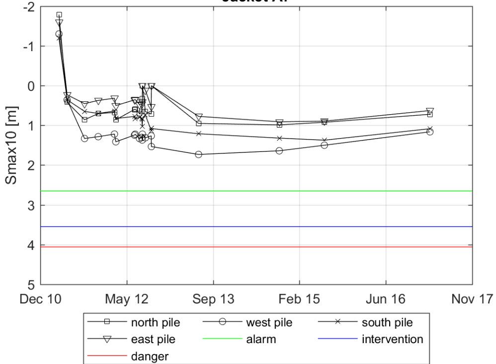
Evolution of Smax10 in a radius of 3m around the pile Jacket A7
