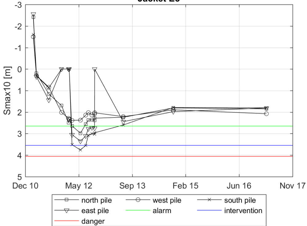
Evolution of Smax10 in a radius of 3m around the pile Jacket E3
