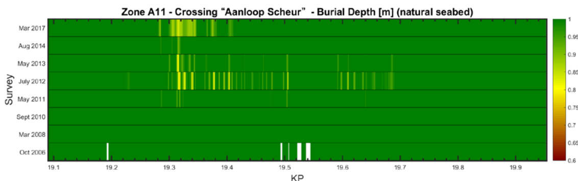
Figure 4-14: Evolution of the Depth of Cover along the cable trajectory along zone A11
