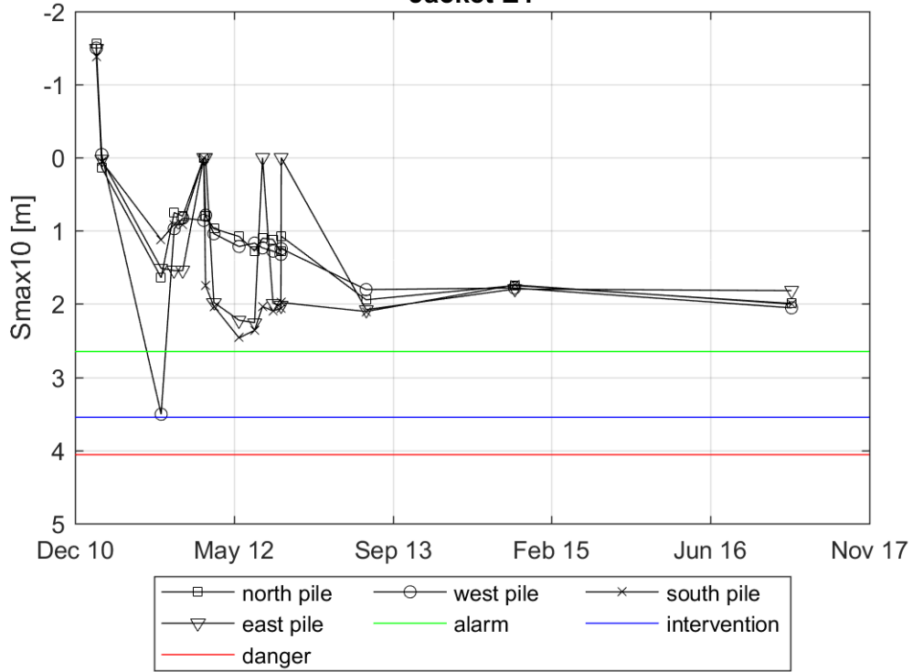
Evolution of Smax10 in a radius of 3m around the pile Jacket E1
