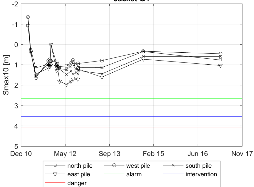
Evolution of Smax10 in a radius of 3m around the pile Jacket G4
