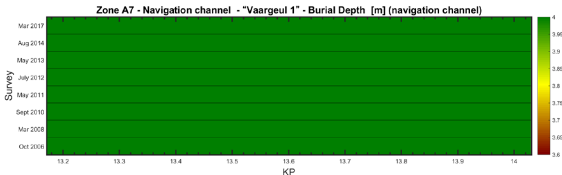
Figure 4-10: Evolution of the Depth of Cover along the cable trajectory along zone A7
