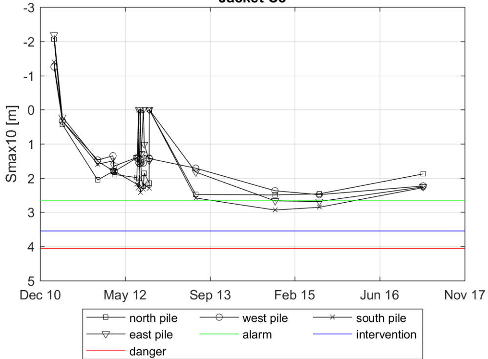
Evolution of Smax10 in a radius of 3m around the pile Jacket C3
