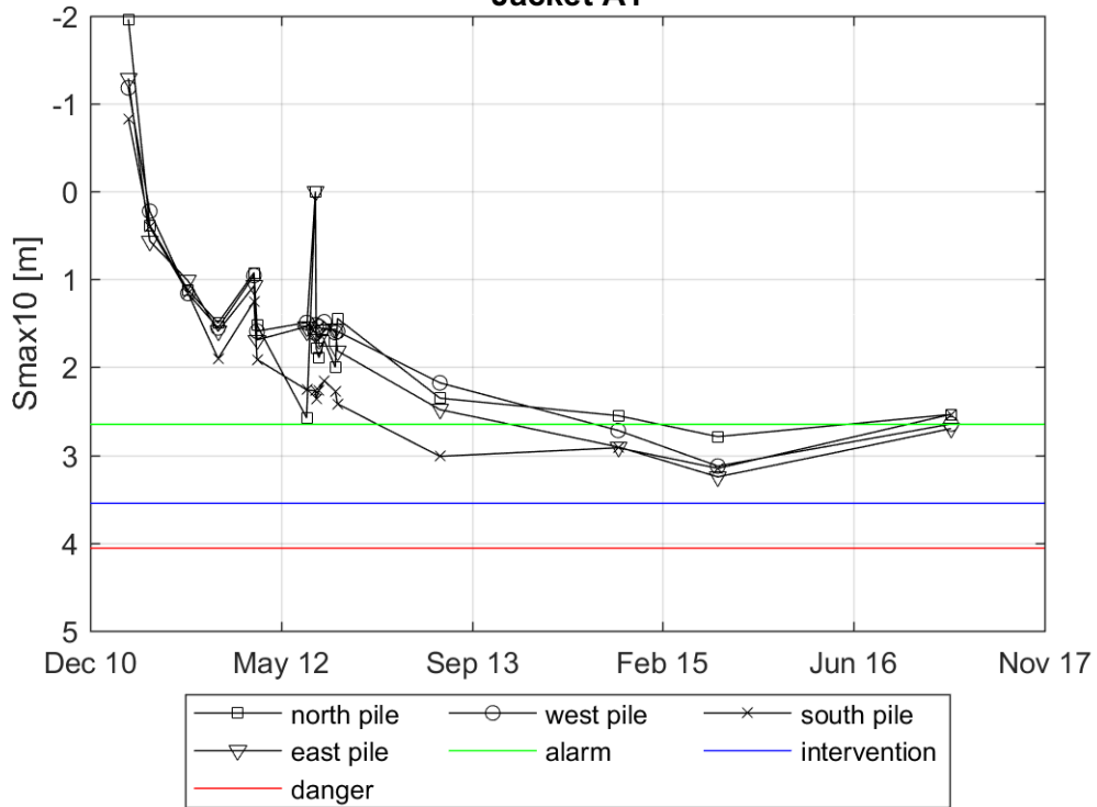
Evolution of Smax10 in a radius of 3m around the pile Jacket A1
