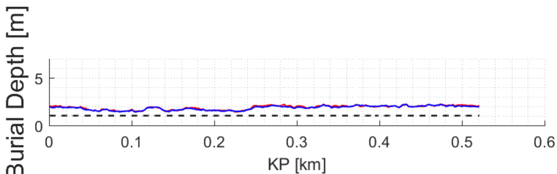
--- Legal burial depth — Survey August 2014 — Survey March 2017
