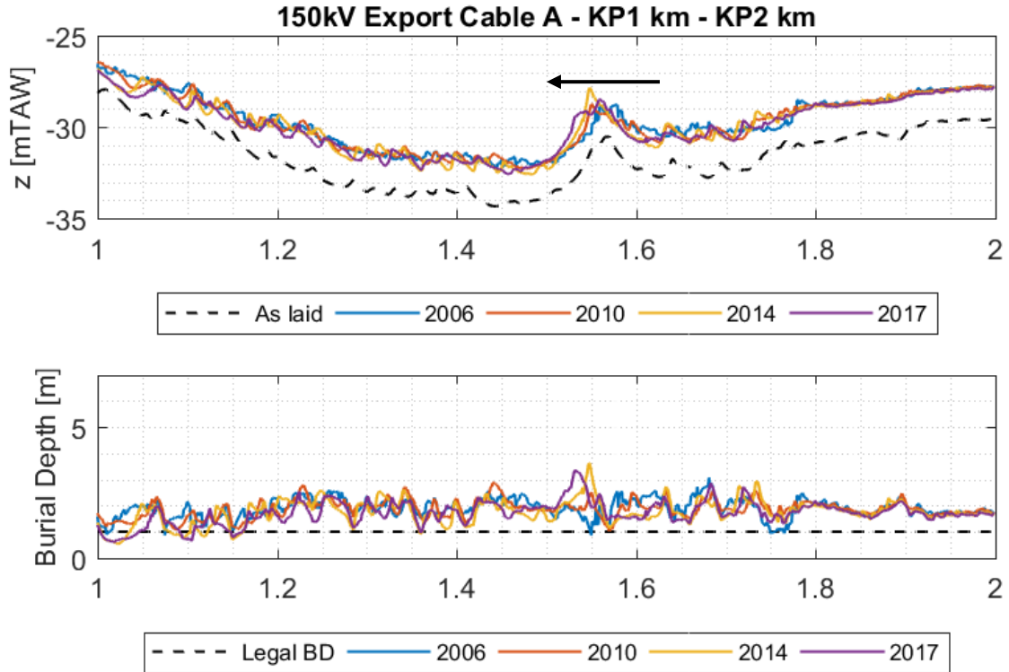
Figure 4-3: Detail of the Depth of Cover along export cable A, zone A2
