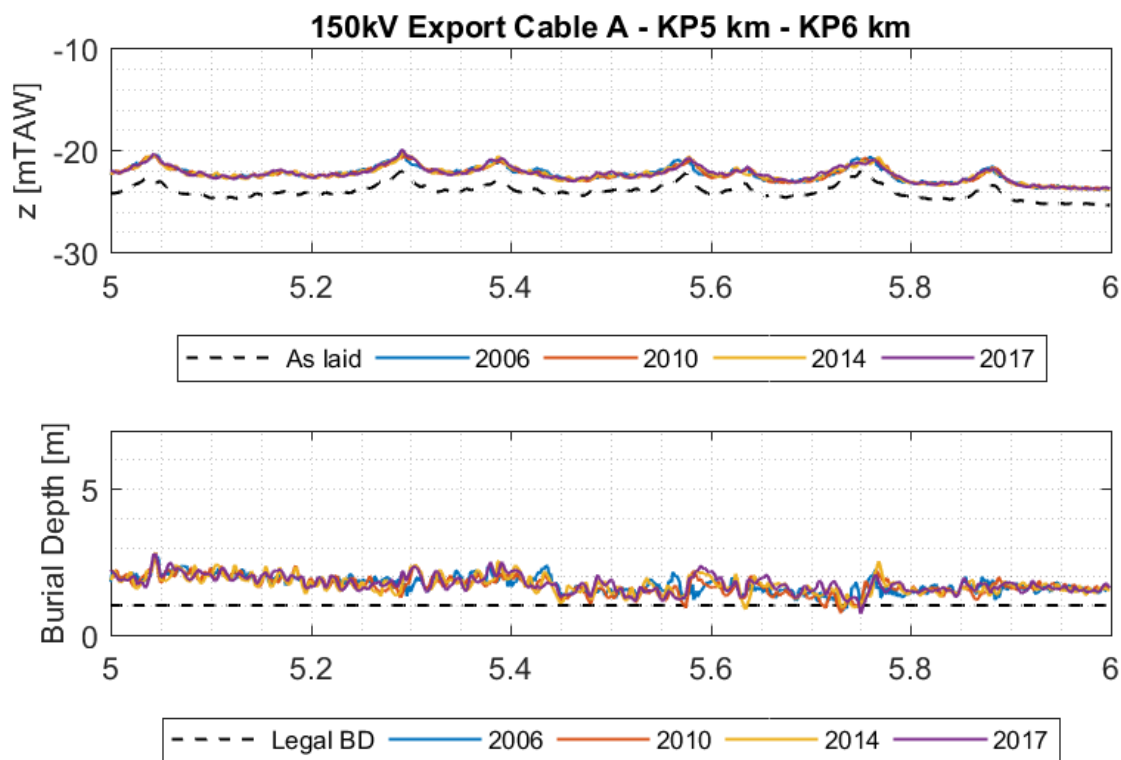
Figure 4-5: Detail of the Depth of Cover along cable A - zone A3)
