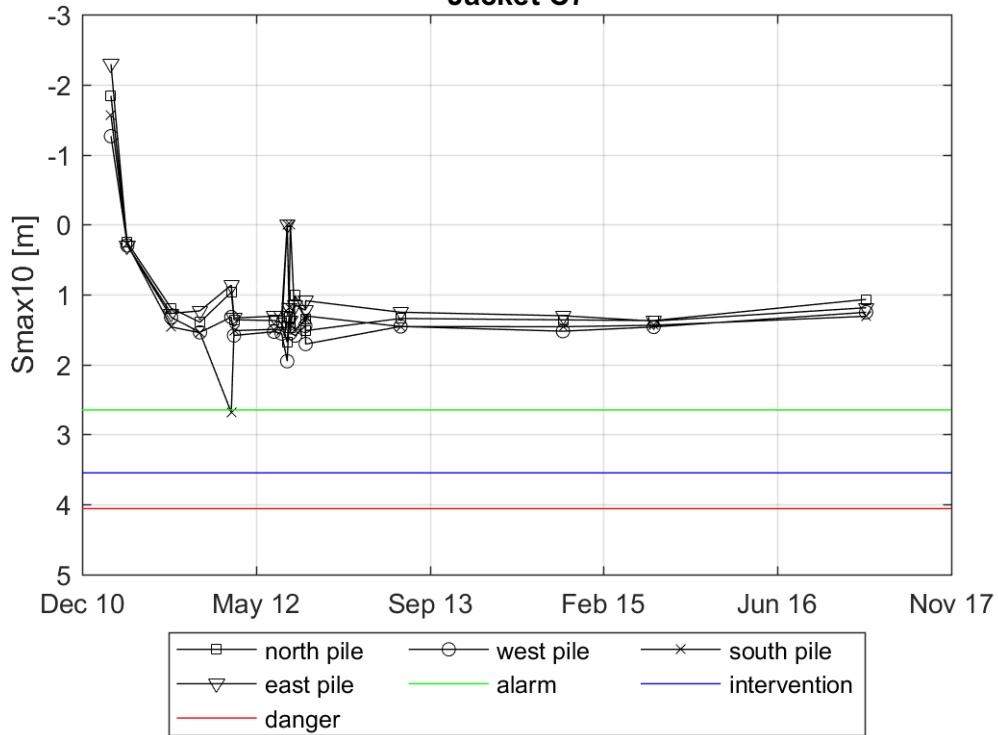
Evolution of Smax10 in a radius of 3m around the pile Jacket C7
