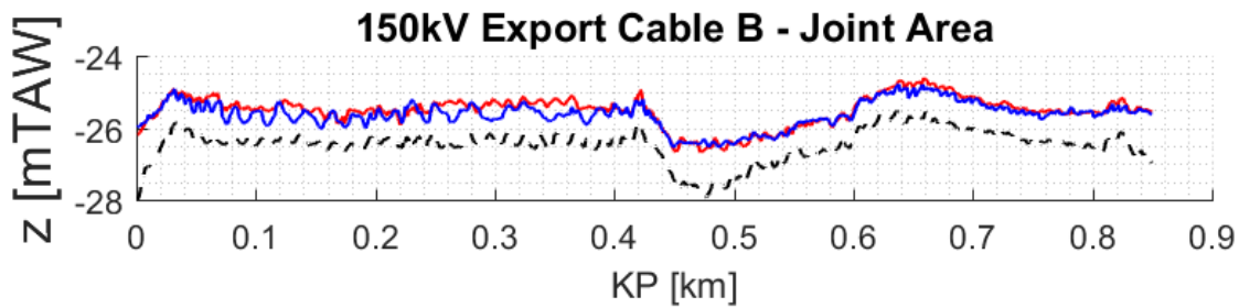
— Top of Aslaid Cable — Survey August 2014 - - - Survey March 2017
