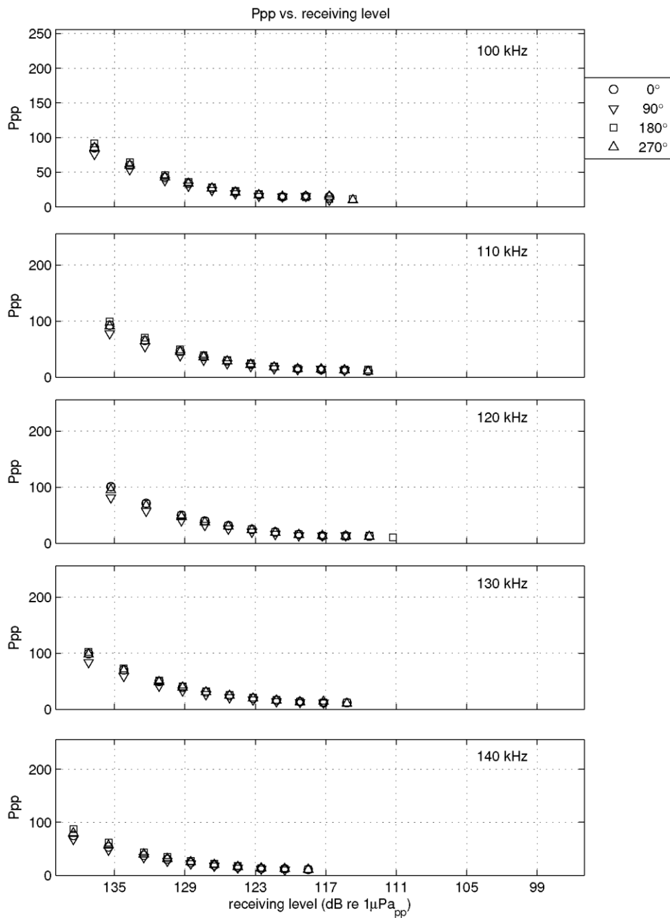
Figure II-21 Calibration results: Ppp vs frequency (this page) and Ppp vs receiving levels (next page) CPOD 3169 after deployment.
