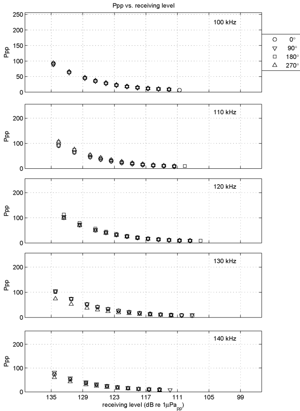
Figure I-14 Calibration results: Ppp vs frequency (this page) and Ppp vs receiving levels (next page) CPOD 1876 before deployment.
