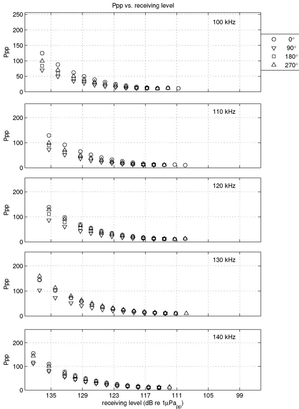
Figure II-10 Calibration results: Ppp vs frequency (this page) and Ppp vs receiving levels (next page) CPOD 1747 after deployment.
