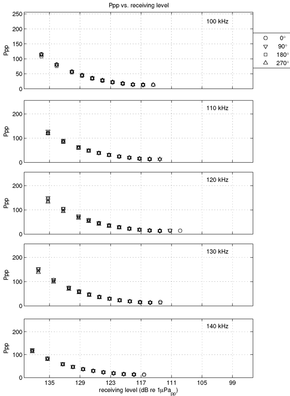
Figure II-1 Calibration results: Ppp vs frequency (this page) and Ppp vs receiving levels (next page) CPOD 376 after deployment.
