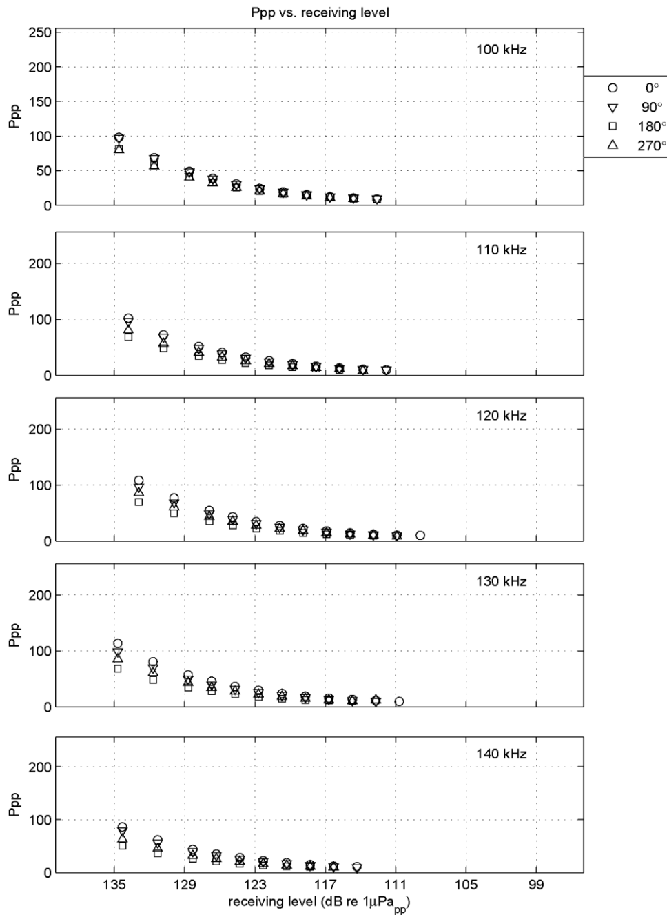
Figure I-22 Calibration results: Ppp vs frequency (this page) and Ppp vs receiving levels (next page) CPOD 3175 before deployment.
