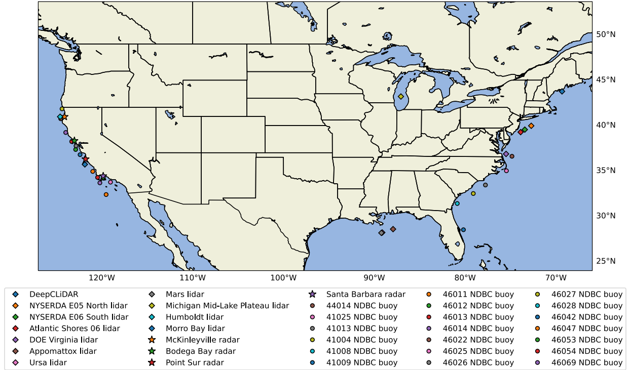
Figure 3. Map of the observational data sets used to validate the NOW-23 data set. Taken from Bodini et al. (in review).
