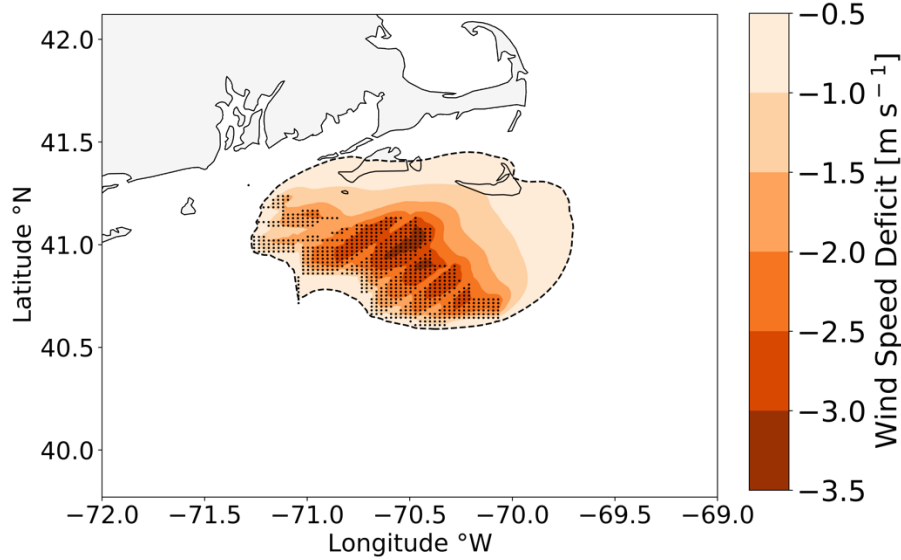
Figure 9. Mean wake wind speeds from the lease areas, for stable conditions, as seen in NOW-WAKES. The wind speed deficit is shown by the colored contour, and the turbines are shown as black dots. The 0.5 \text{ m s}^{-1} deficit is shown by the dotted black line. Taken from Rosencrans et al. (in review).
