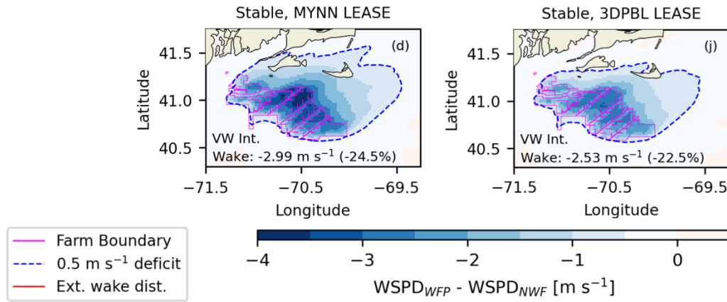
Figure 10. Mean wake wind speed deficit from the lease areas, for stable conditions, using the MYNN PBL scheme (left) and the NCAR 3DPBL scheme (right), at 138 m asl.
