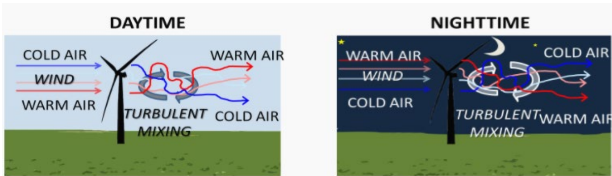
Figure 3. Mixing of Air Layers – Day and Night (Cervarich, 2021)
