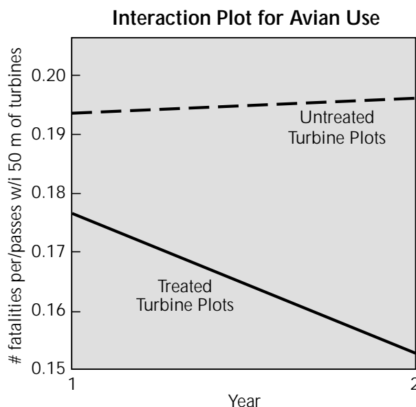
Figure 4-1. Interaction between the number of fatalities per bird passes within 50 meters of treated and untreated turbines.
